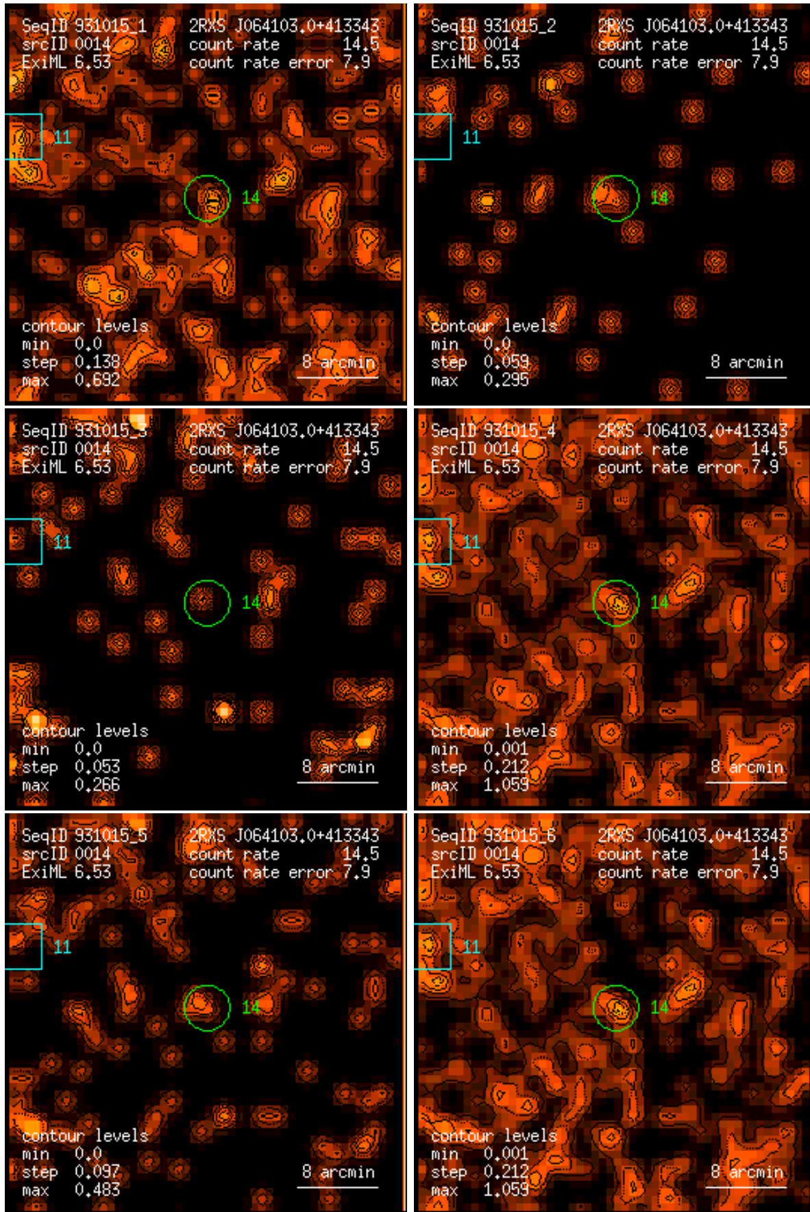
Figure 14: RASS 931015: detection 0014: band rate images, Gaussian filter: (1) PSPC channels 11 – 41, (2) 52 – 90, (3) 91 – 201, (4) 11 – 235, (5) 52 – 201, (6) 11 – 201. Broad band rates in counts/ks. Band rate contour levels in counts/ks/arcmin 2 .
