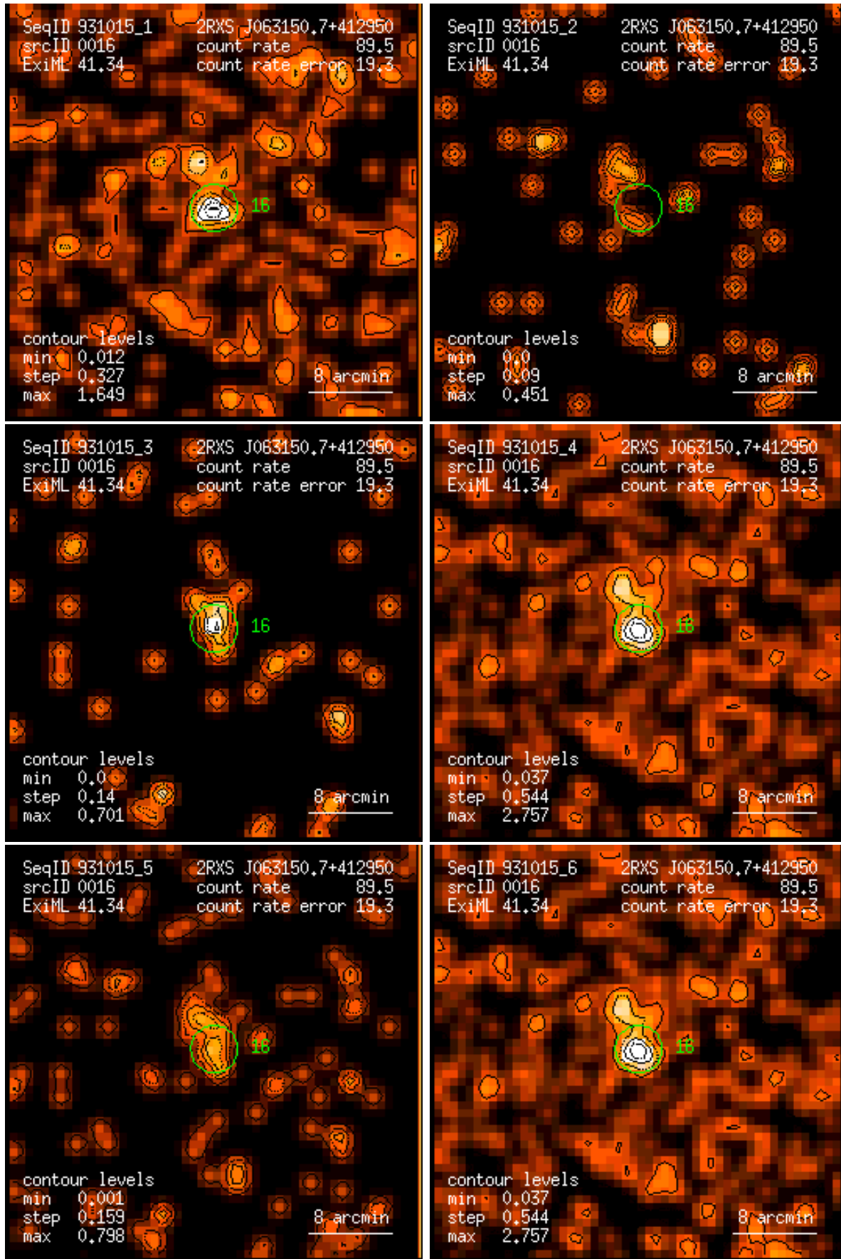
Figure 16: RASS 931015: detection 0016: band rate images, Gaussian filter: (1) PSPC channels 11 – 41, (2) 52 – 90, (3) 91 – 201, (4) 11 – 235, (5) 52 – 201, (6) 11 – 201. Broad band rates in counts/ks. Band rate contour levels in counts/ks/arcmin 2 .
