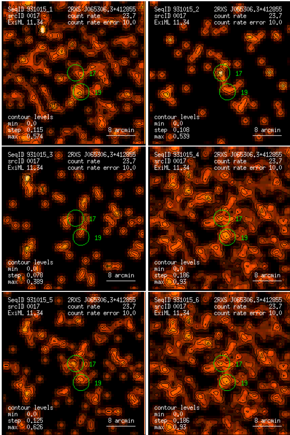
Figure 17: RASS 931015: detection 0017: band rate images, Gaussian filter: (1) PSPC channels 11 – 41, (2) 52 – 90, (3) 91 – 201, (4) 11 – 235, (5) 52 – 201, (6) 11 – 201. Broad band rates in counts/ks. Band rate contour levels in counts/ks/arcmin 2 .
