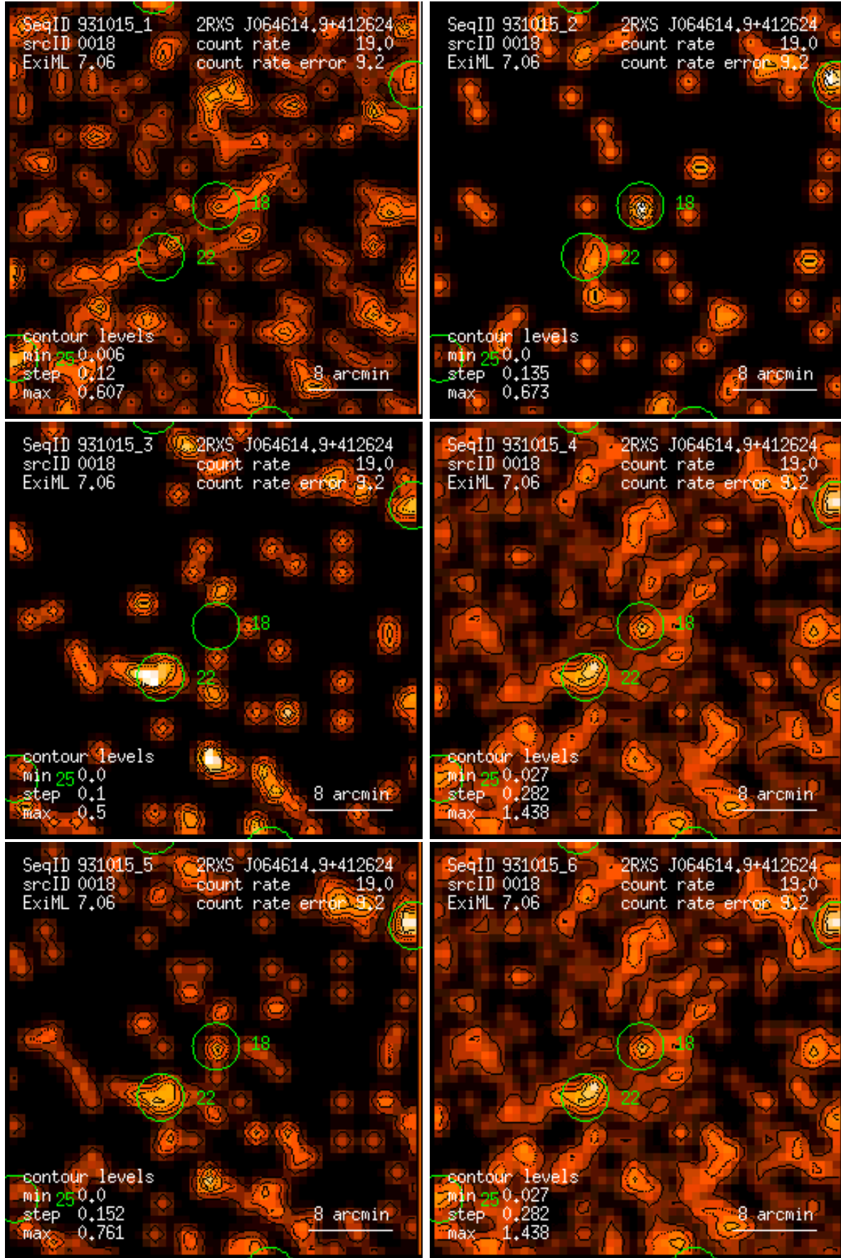
Figure 18: RASS 931015: detection 0018: band rate images, Gaussian filter: (1) PSPC channels 11 – 41, (2) 52 – 90, (3) 91 – 201, (4) 11 – 235, (5) 52 – 201, (6) 11 – 201. Broad band rates in counts/ks. Band rate contour levels in counts/ks/arcmin 2 .
