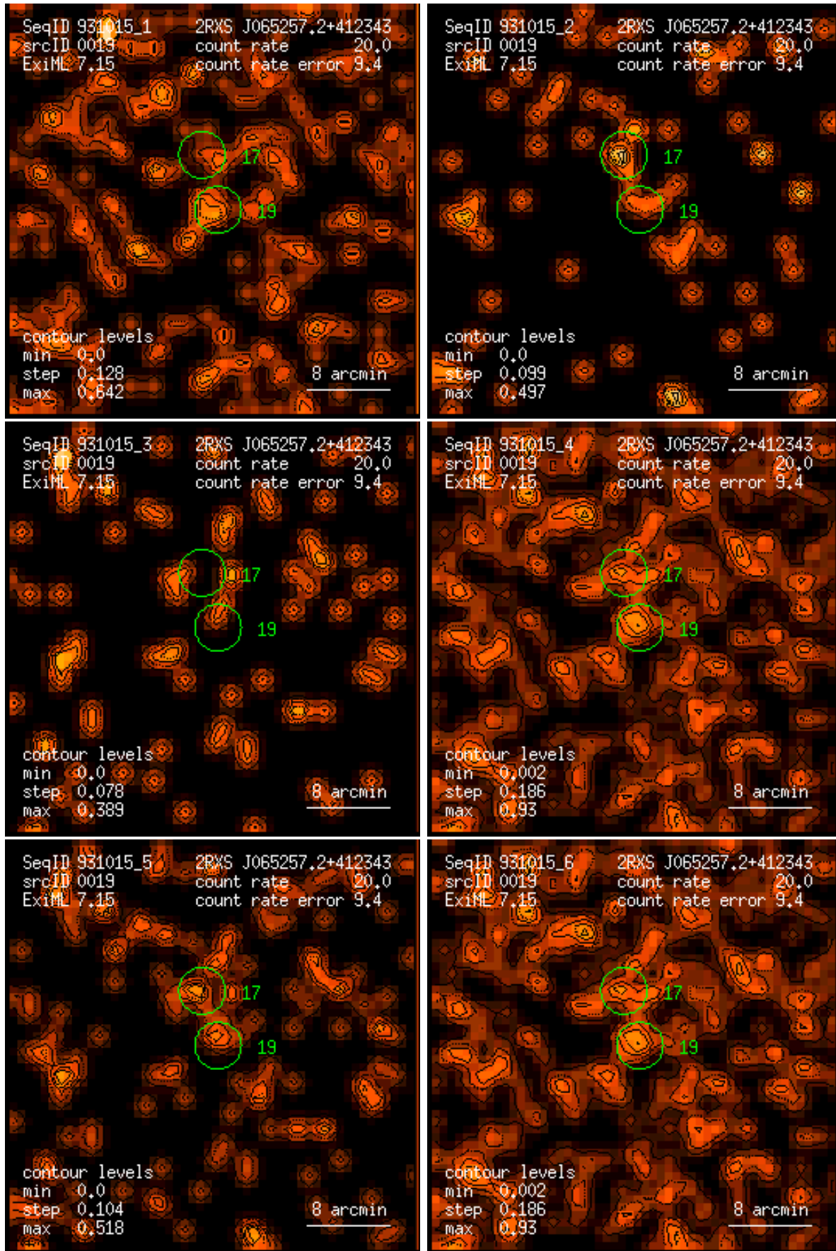
Figure 19: RASS 931015: detection 0019: band rate images, Gaussian filter: (1) PSPC channels 11 – 41, (2) 52 – 90, (3) 91 – 201, (4) 11 – 235, (5) 52 – 201, (6) 11 – 201. Broad band rates in counts/ks. Band rate contour levels in counts/ks/arcmin 2 .
