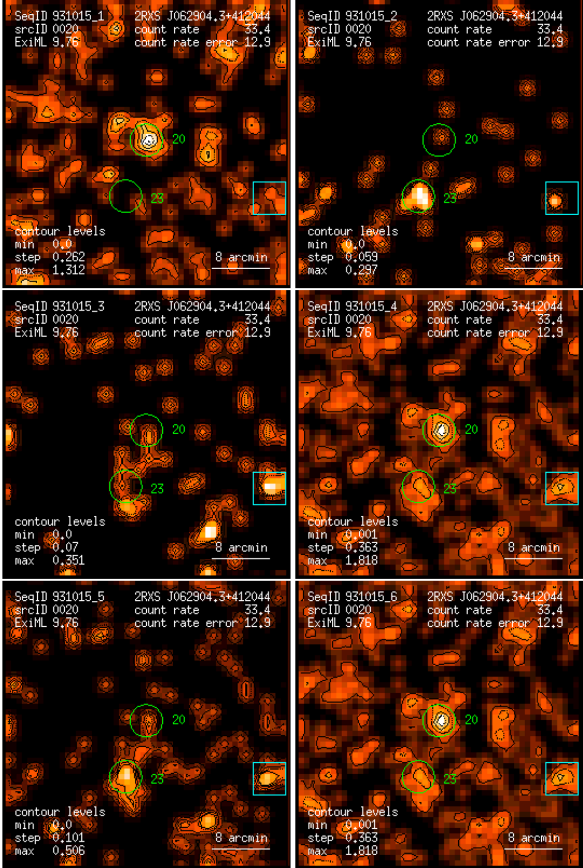
Figure 20: RASS 931015: detection 0020: band rate images, Gaussian filter: (1) PSPC channels 11 – 41, (2) 52 – 90, (3) 91 – 201, (4) 11 – 235, (5) 52 – 201, (6) 11 – 201. Broad band rates in counts/ks. Band rate contour levels in counts/ks/arcmin 2 .
