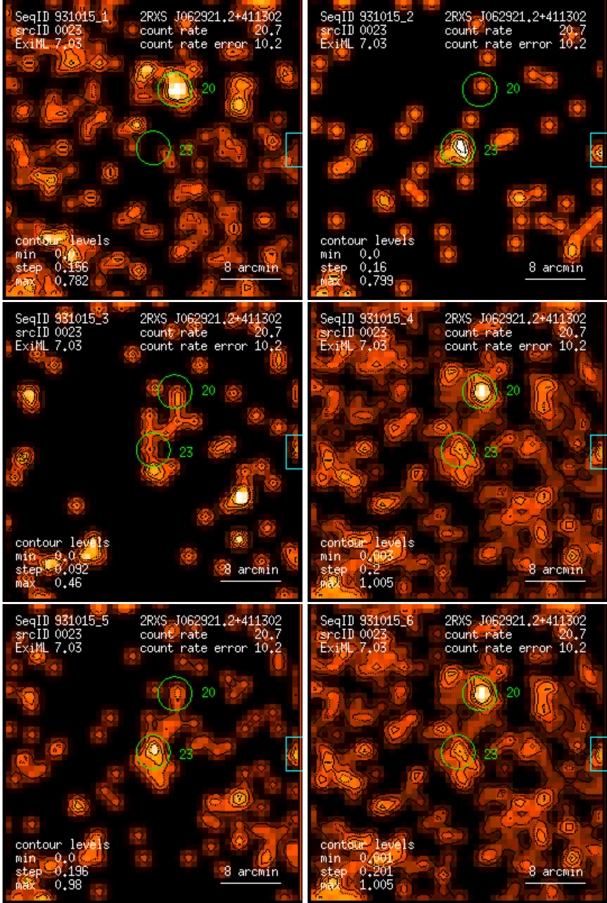
Figure 23: RASS 931015: detection 0023: band rate images, Gaussian filter: (1) PSPC channels 11 – 41, (2) 52 – 90, (3) 91 – 201, (4) 11 – 235, (5) 52 – 201, (6) 11 – 201. Broad band rates in counts/ks. Band rate contour levels in counts/ks/arcmin 2 .
