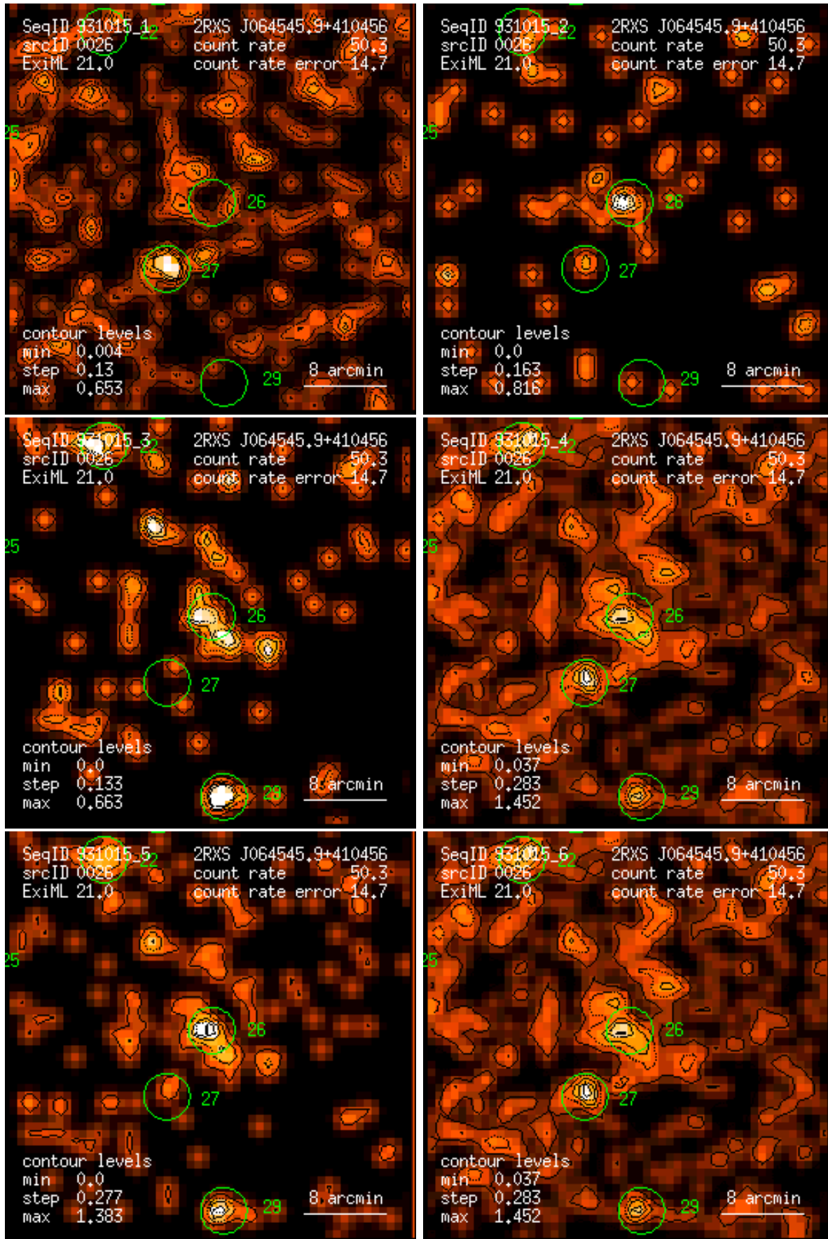
Figure 26: RASS 931015: detection 0026: band rate images, Gaussian filter: (1) PSPC channels 11 – 41, (2) 52 – 90, (3) 91 – 201, (4) 11 – 235, (5) 52 – 201, (6) 11 – 201. Broad band rates in counts/ks. Band rate contour levels in counts/ks/arcmin 2 .
