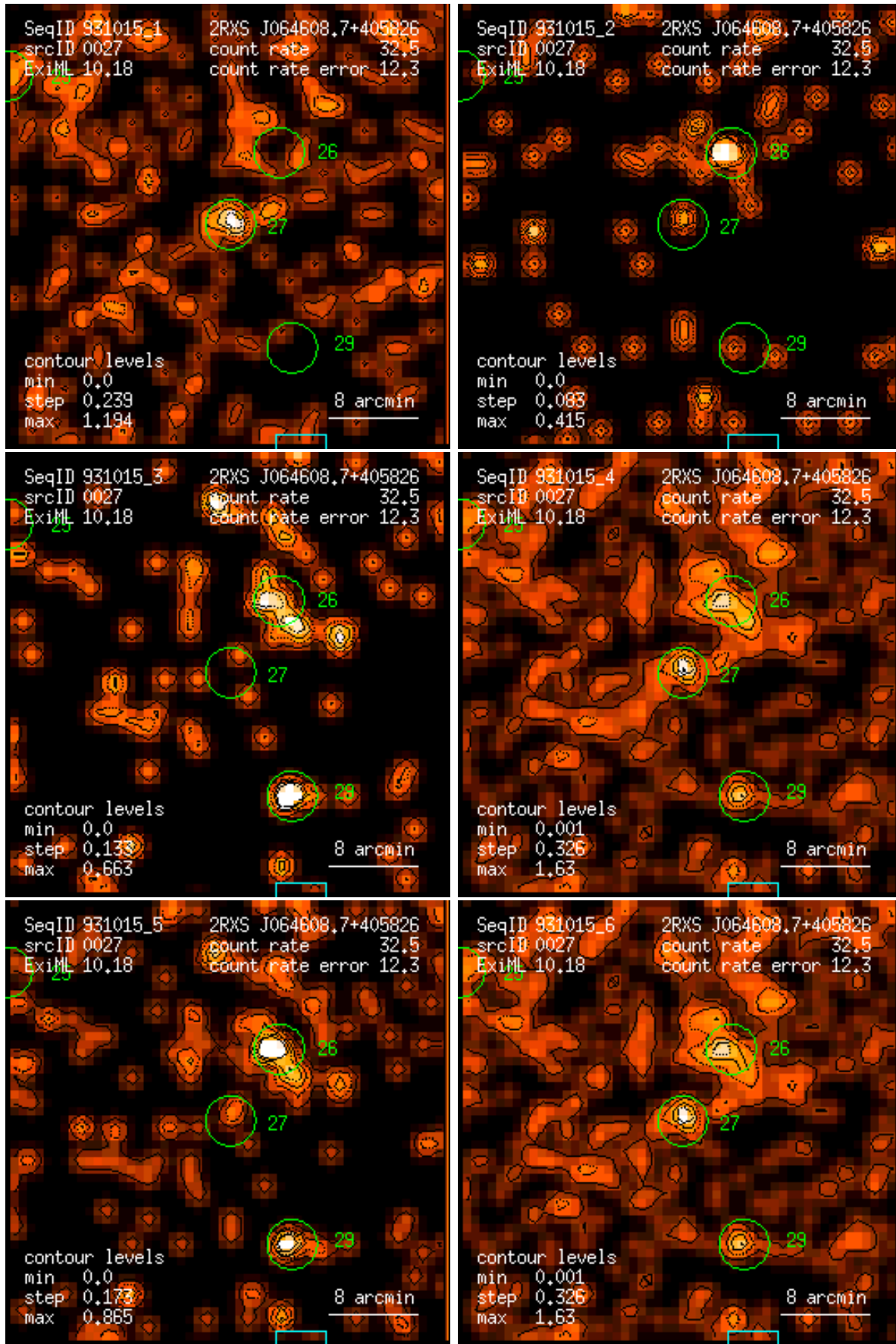
Figure 27: RASS 931015: detection 0027: band rate images, Gaussian filter: (1) PSPC channels 11 – 41, (2) 52 – 90, (3) 91 – 201, (4) 11 – 235, (5) 52 – 201, (6) 11 – 201. Broad band rates in counts/ks. Band rate contour levels in counts/ks/arcmin 2 .
