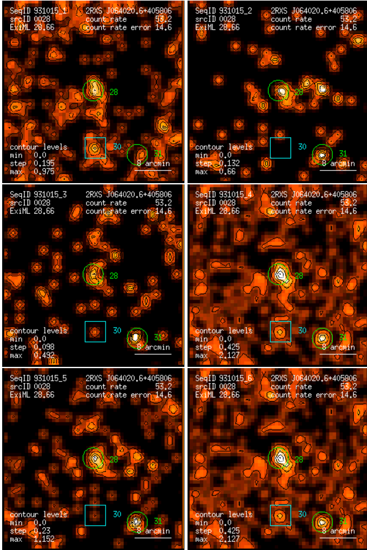
Figure 28: RASS 931015: detection 0028: band rate images, Gaussian filter: (1) PSPC channels 11 – 41, (2) 52 – 90, (3) 91 – 201, (4) 11 – 235, (5) 52 – 201, (6) 11 – 201. Broad band rates in counts/ks. Band rate contour levels in counts/ks/arcmin 2 .
