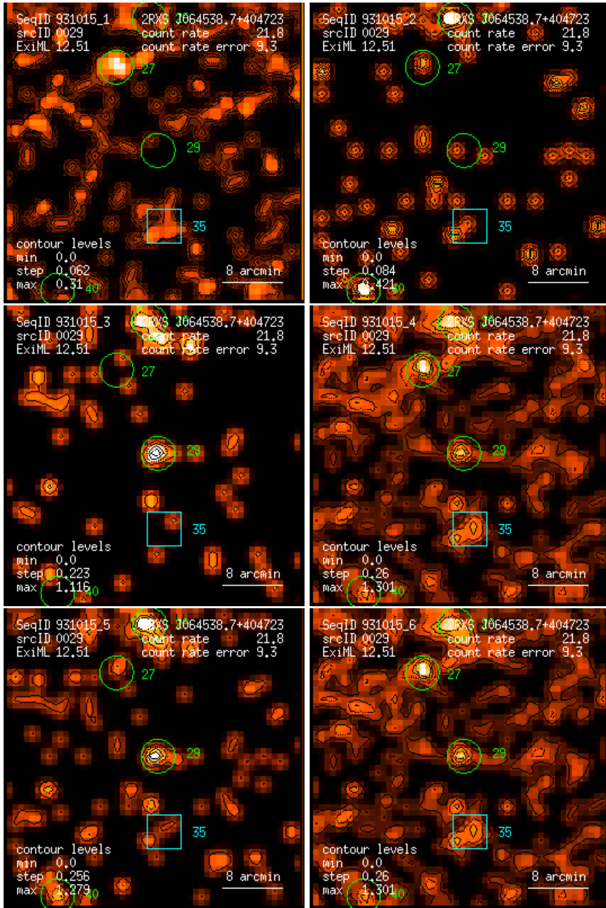
Figure 29: RASS 931015: detection 0029: band rate images, Gaussian filter: (1) PSPC channels 11 – 41, (2) 52 – 90, (3) 91 – 201, (4) 11 – 235, (5) 52 – 201, (6) 11 – 201. Broad band rates in counts/ks. Band rate contour levels in counts/ks/arcmin 2 .
