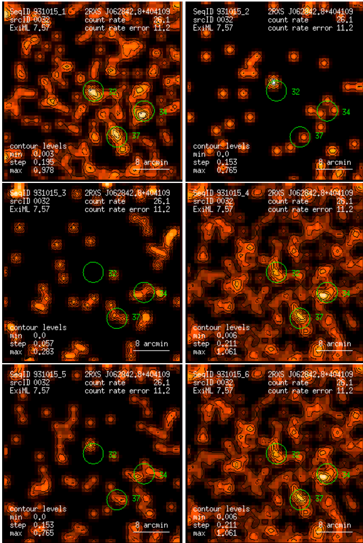
Figure 32: RASS 931015: detection 0032: band rate images, Gaussian filter: (1) PSPC channels 11 – 41, (2) 52 – 90, (3) 91 – 201, (4) 11 – 235, (5) 52 – 201, (6) 11 – 201. Broad band rates in counts/ks. Band rate contour levels in counts/ks/arcmin 2 .
