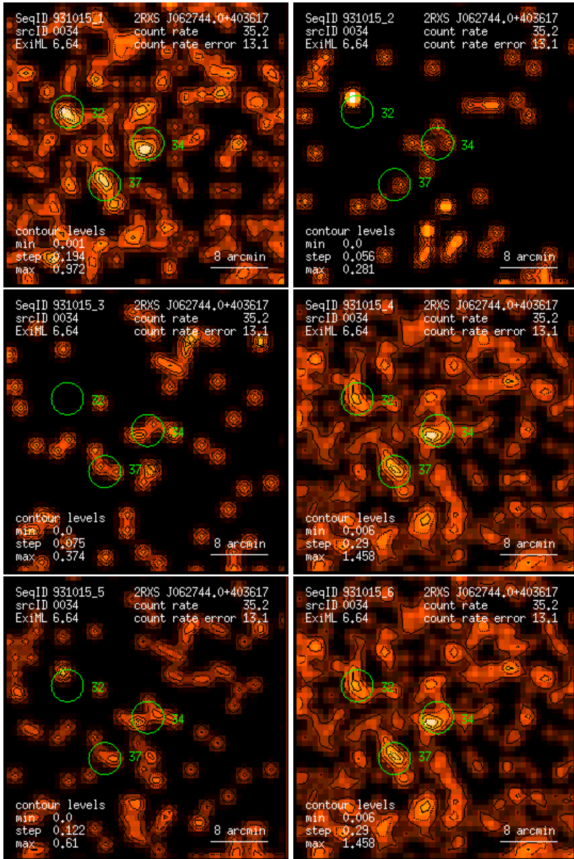
Figure 34: RASS 931015: detection 0034: band rate images, Gaussian filter: (1) PSPC channels 11 – 41, (2) 52 – 90, (3) 91 – 201, (4) 11 – 235, (5) 52 – 201, (6) 11 – 201. Broad band rates in counts/ks. Band rate contour levels in counts/ks/arcmin 2 .
