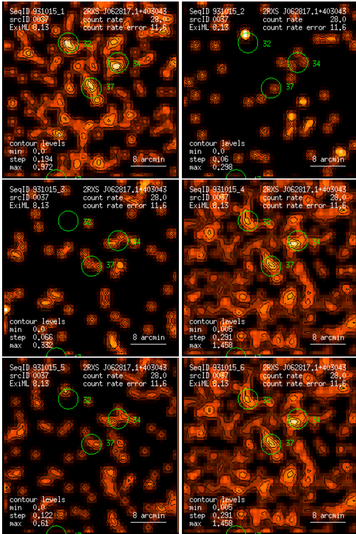
Figure 37: RASS 931015: detection 0037: band rate images, Gaussian filter: (1) PSPC channels 11 – 41, (2) 52 – 90, (3) 91 – 201, (4) 11 – 235, (5) 52 – 201, (6) 11 – 201. Broad band rates in counts/ks. Band rate contour levels in counts/ks/arcmin 2 .
