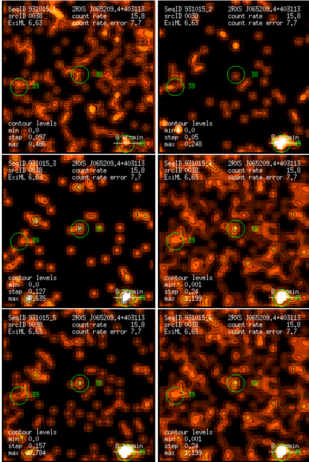
Figure 38: RASS 931015: detection 0038: band rate images, Gaussian filter: (1) PSPC channels 11 – 41, (2) 52 – 90, (3) 91 – 201, (4) 11 – 235, (5) 52 – 201, (6) 11 – 201. Broad band rates in counts/ks. Band rate contour levels in counts/ks/arcmin 2 .
