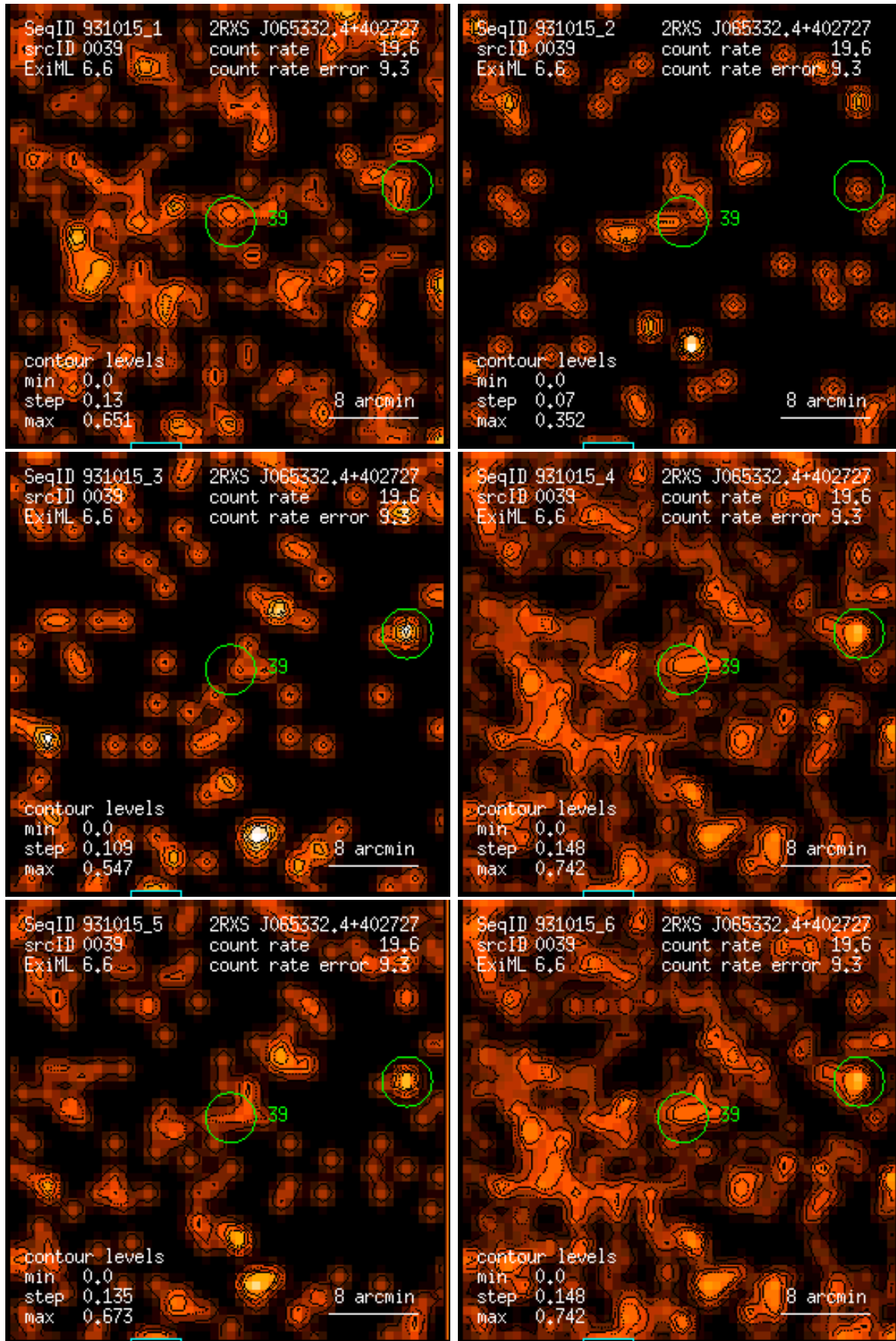
Figure 39: RASS 931015: detection 0039: band rate images, Gaussian filter: (1) PSPC channels 11 – 41, (2) 52 – 90, (3) 91 – 201, (4) 11 – 235, (5) 52 – 201, (6) 11 – 201. Broad band rates in counts/ks. Band rate contour levels in counts/ks/arcmin 2 .
