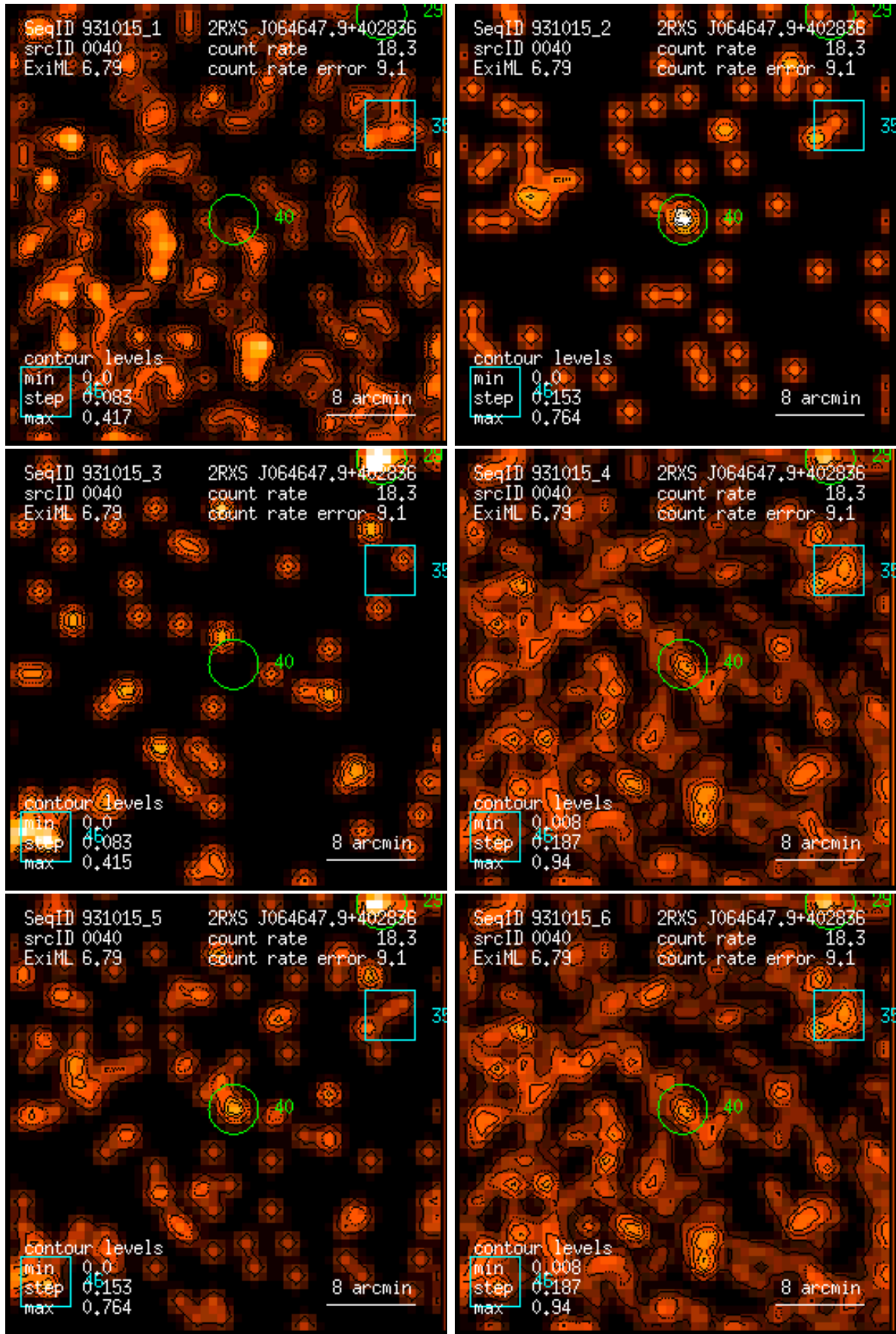
Figure 40: RASS 931015: detection 0040: band rate images, Gaussian filter: (1) PSPC channels 11 – 41, (2) 52 – 90, (3) 91 – 201, (4) 11 – 235, (5) 52 – 201, (6) 11 – 201. Broad band rates in counts/ks. Band rate contour levels in counts/ks/arcmin 2 .
