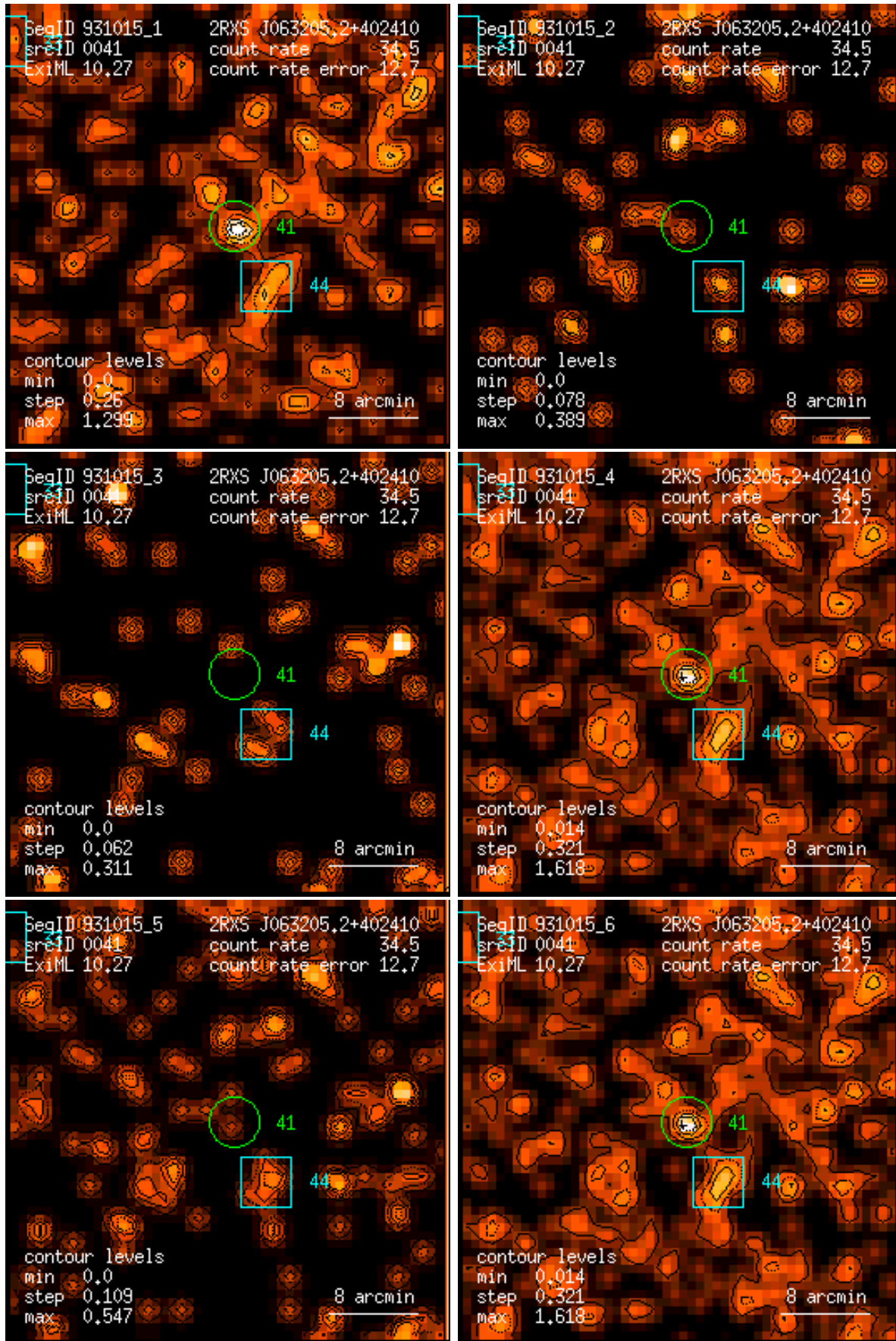
Figure 41: RASS 931015: detection 0041: band rate images, Gaussian filter: (1) PSPC channels 11 – 41, (2) 52 – 90, (3) 91 – 201, (4) 11 – 235, (5) 52 – 201, (6) 11 – 201. Broad band rates in counts/ks. Band rate contour levels in counts/ks/arcmin 2 .
