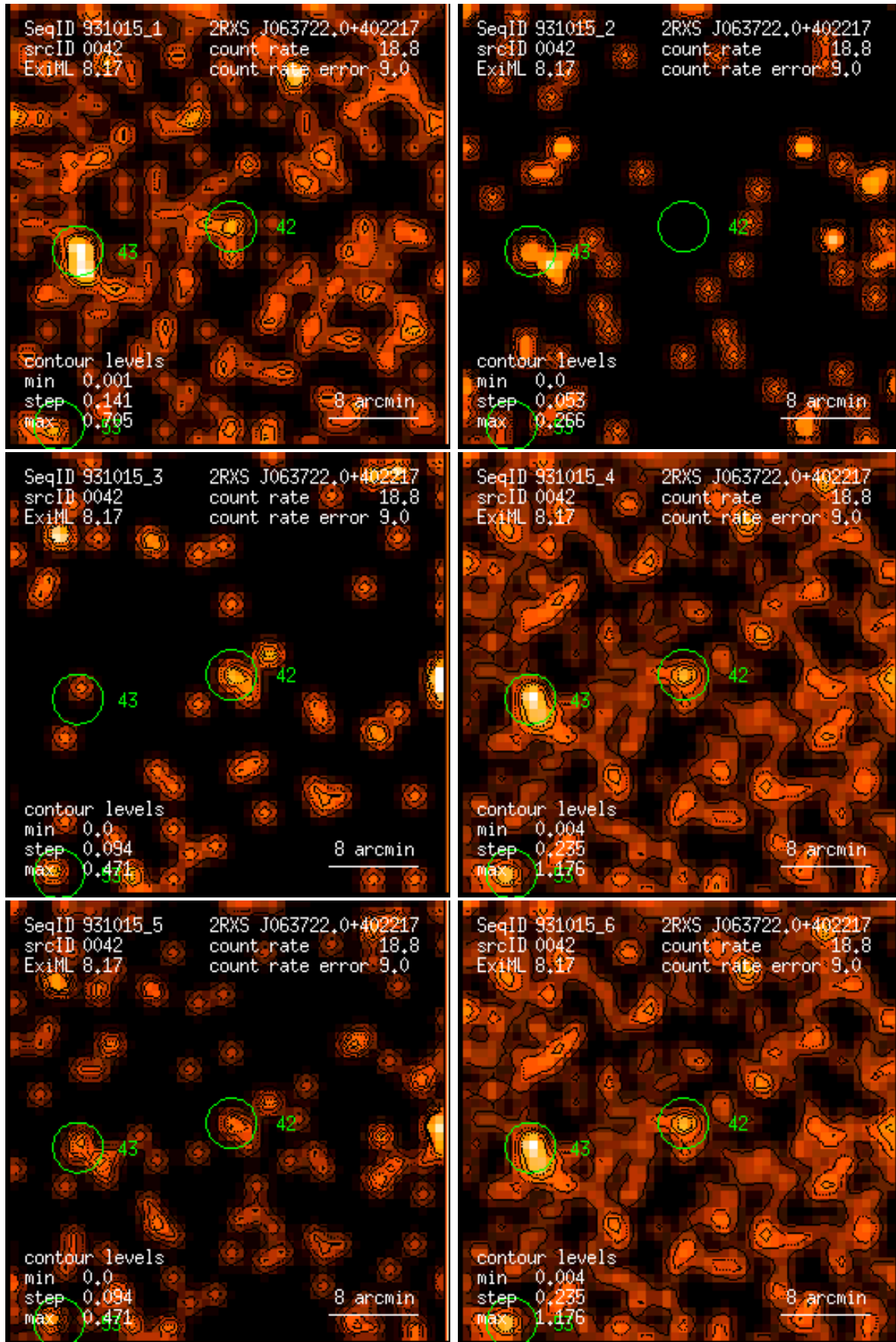
Figure 42: RASS 931015: detection 0042: band rate images, Gaussian filter: (1) PSPC channels 11 – 41, (2) 52 – 90, (3) 91 – 201, (4) 11 – 235, (5) 52 – 201, (6) 11 – 201. Broad band rates in counts/ks. Band rate contour levels in counts/ks/arcmin 2 .
