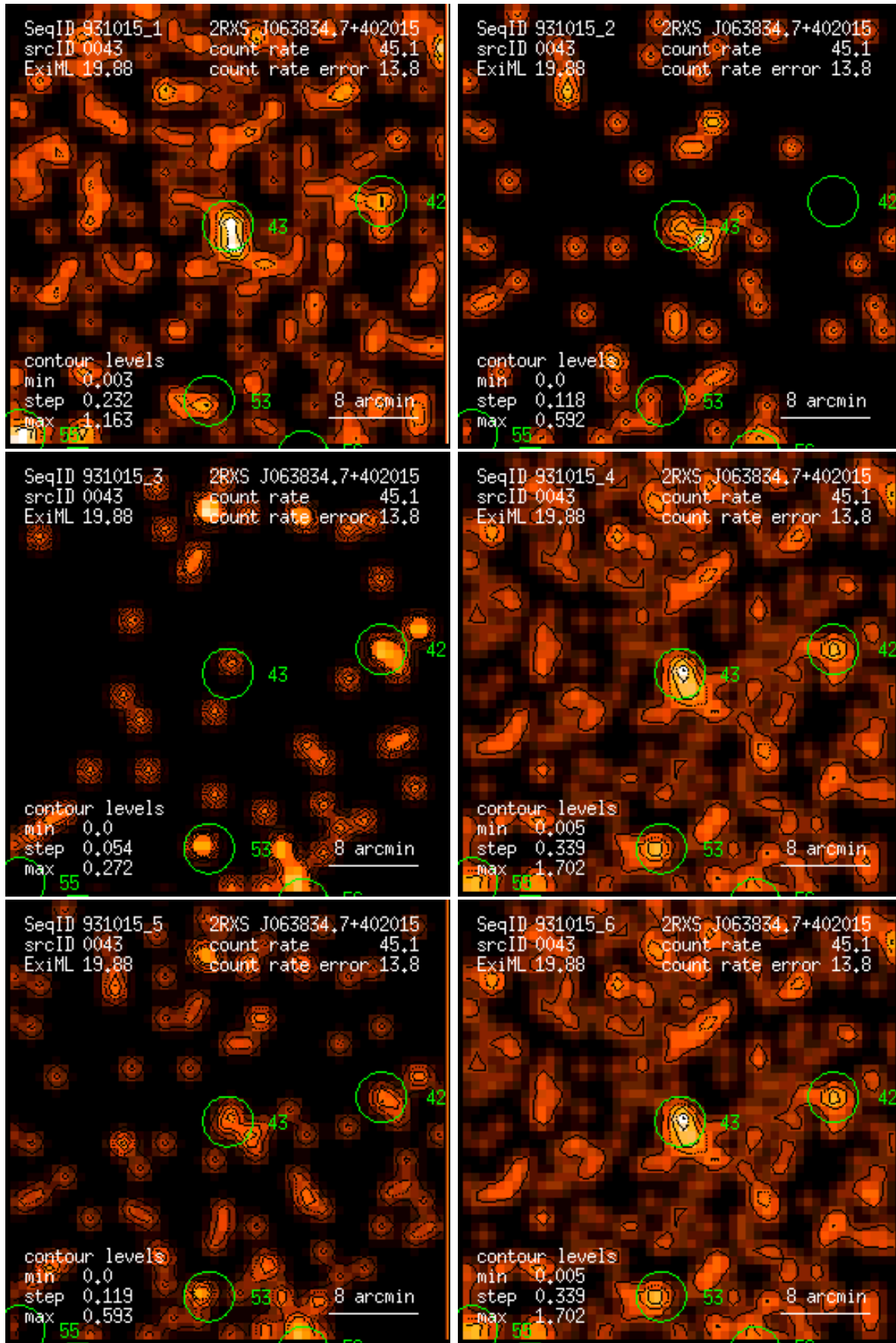
Figure 43: RASS 931015: detection 0043: band rate images, Gaussian filter: (1) PSPC channels 11 – 41, (2) 52 – 90, (3) 91 – 201, (4) 11 – 235, (5) 52 – 201, (6) 11 – 201. Broad band rates in counts/ks. Band rate contour levels in counts/ks/arcmin 2 .
