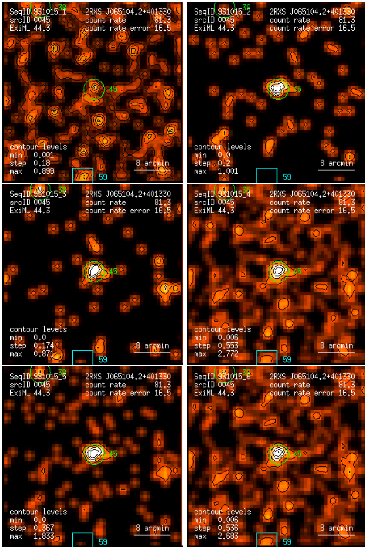
Figure 45: RASS 931015: detection 0045: band rate images, Gaussian filter: (1) PSPC channels 11 – 41, (2) 52 – 90, (3) 91 – 201, (4) 11 – 235, (5) 52 – 201, (6) 11 – 201. Broad band rates in counts/ks. Band rate contour levels in counts/ks/arcmin 2 .
