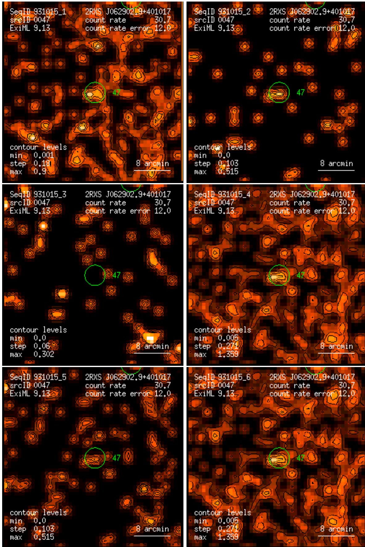
Figure 47: RASS 931015: detection 0047: band rate images, Gaussian filter: (1) PSPC channels 11 – 41, (2) 52 – 90, (3) 91 – 201, (4) 11 – 235, (5) 52 – 201, (6) 11 – 201. Broad band rates in counts/ks. Band rate contour levels in counts/ks/arcmin 2 .
