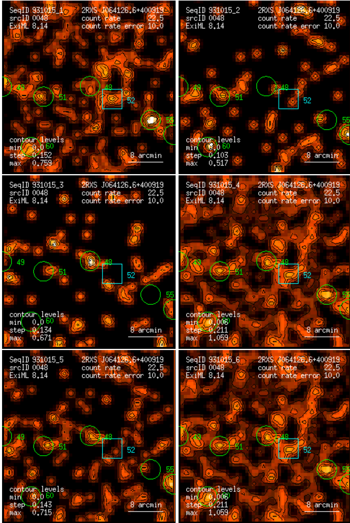
Figure 48: RASS 931015: detection 0048: band rate images, Gaussian filter: (1) PSPC channels 11 – 41, (2) 52 – 90, (3) 91 – 201, (4) 11 – 235, (5) 52 – 201, (6) 11 – 201. Broad band rates in counts/ks. Band rate contour levels in counts/ks/arcmin 2 .
