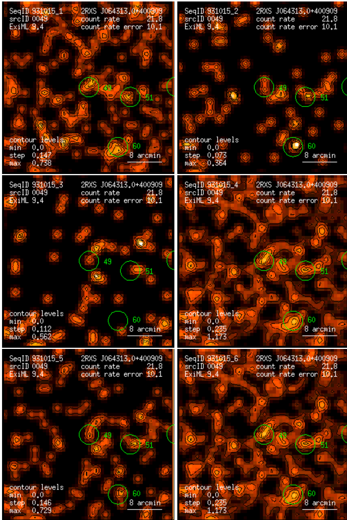
Figure 49: RASS 931015: detection 0049: band rate images, Gaussian filter: (1) PSPC channels 11 – 41, (2) 52 – 90, (3) 91 – 201, (4) 11 – 235, (5) 52 – 201, (6) 11 – 201. Broad band rates in counts/ks. Band rate contour levels in counts/ks/arcmin 2 .
