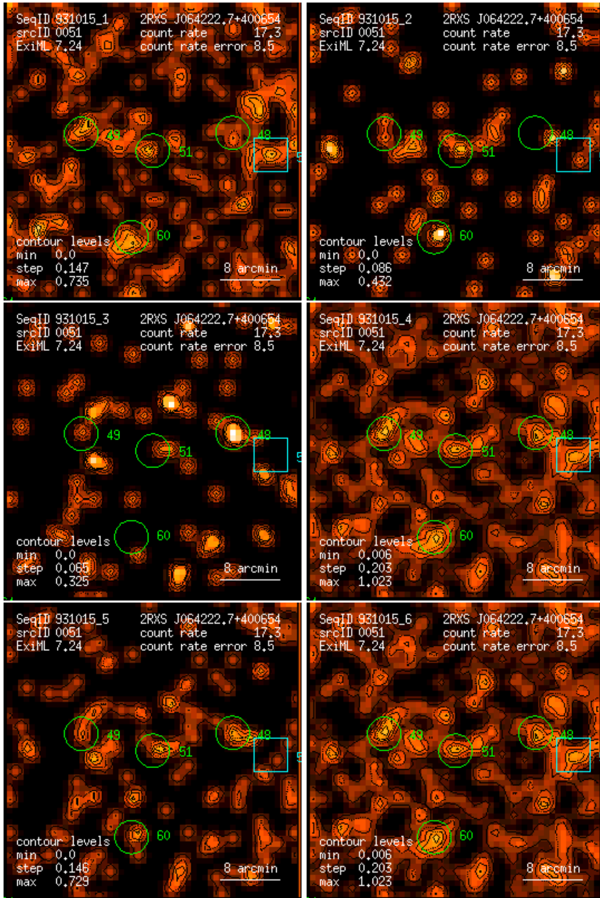
Figure 51: RASS 931015: detection 0051: band rate images, Gaussian filter: (1) PSPC channels 11 – 41, (2) 52 – 90, (3) 91 – 201, (4) 11 – 235, (5) 52 – 201, (6) 11 – 201. Broad band rates in counts/ks. Band rate contour levels in counts/ks/arcmin 2 .
