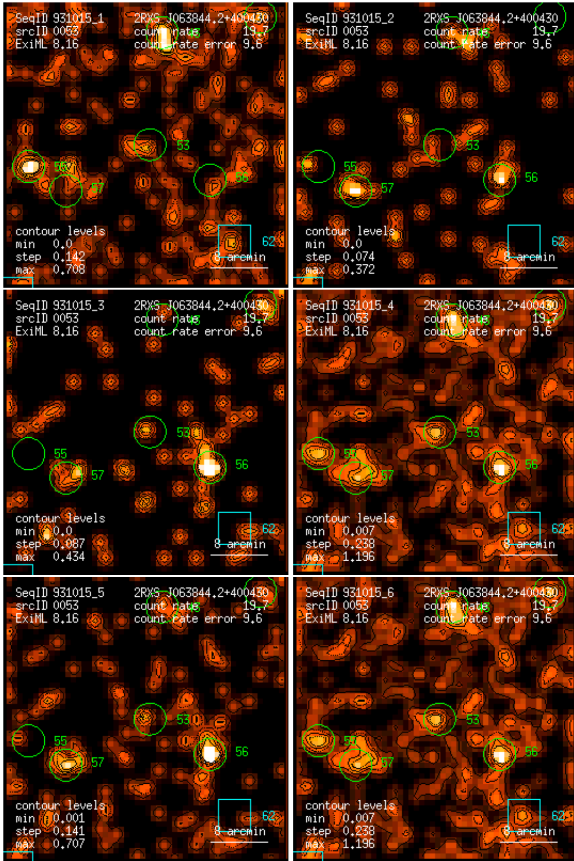
Figure 53: RASS 931015: detection 0053: band rate images, Gaussian filter: (1) PSPC channels 11 – 41, (2) 52 – 90, (3) 91 – 201, (4) 11 – 235, (5) 52 – 201, (6) 11 – 201. Broad band rates in counts/ks. Band rate contour levels in counts/ks/arcmin 2 .
