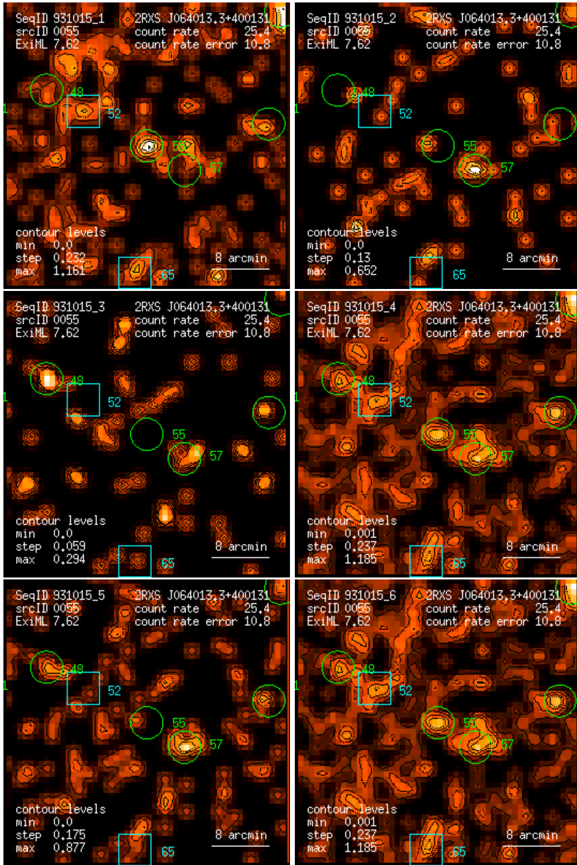
Figure 55: RASS 931015: detection 0055: band rate images, Gaussian filter: (1) PSPC channels 11 – 41, (2) 52 – 90, (3) 91 – 201, (4) 11 – 235, (5) 52 – 201, (6) 11 – 201. Broad band rates in counts/ks. Band rate contour levels in counts/ks/arcmin 2 .
