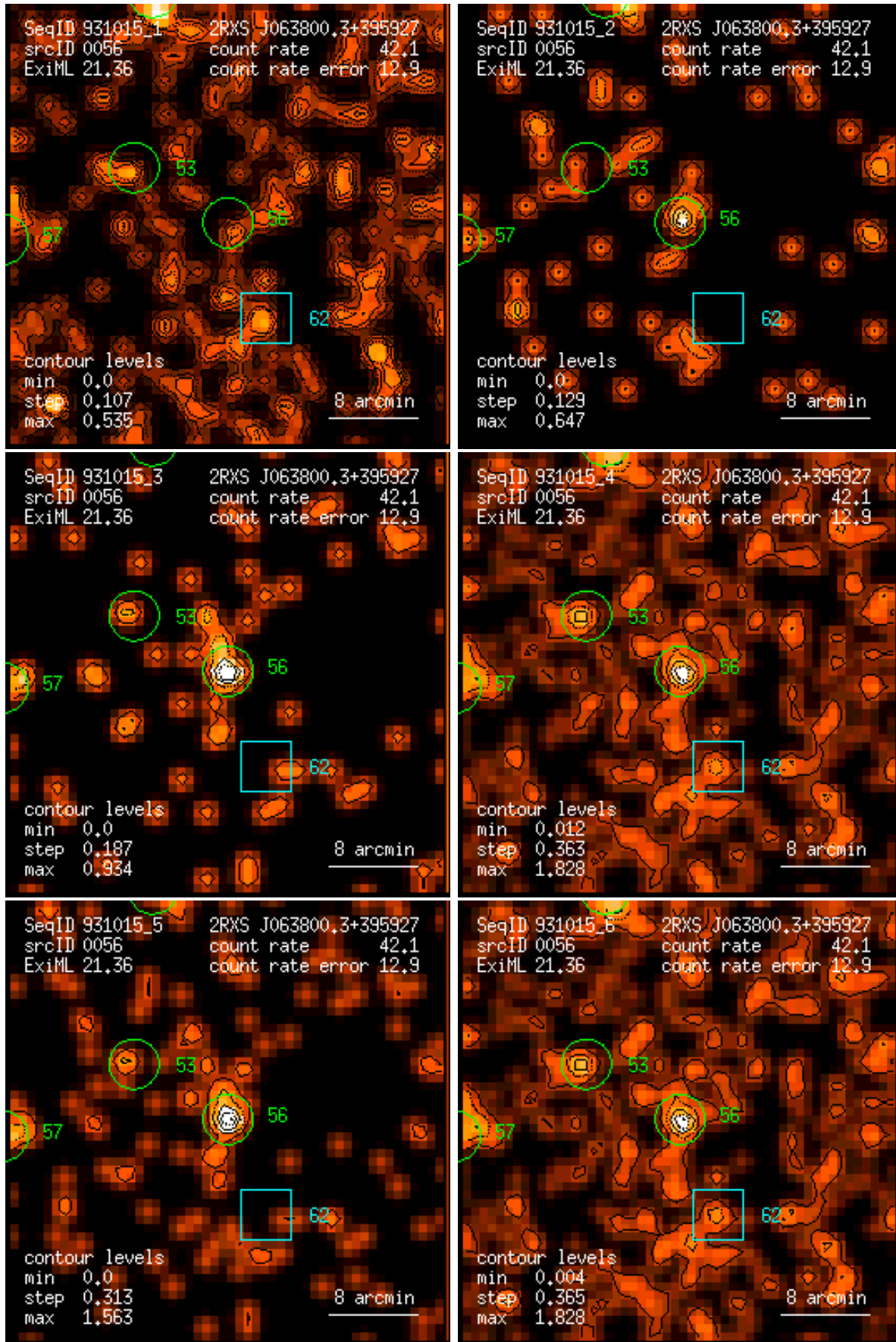
Figure 56: RASS 931015: detection 0056: band rate images, Gaussian filter: (1) PSPC channels 11 – 41, (2) 52 – 90, (3) 91 – 201, (4) 11 – 235, (5) 52 – 201, (6) 11 – 201. Broad band rates in counts/ks. Band rate contour levels in counts/ks/arcmin 2 .
