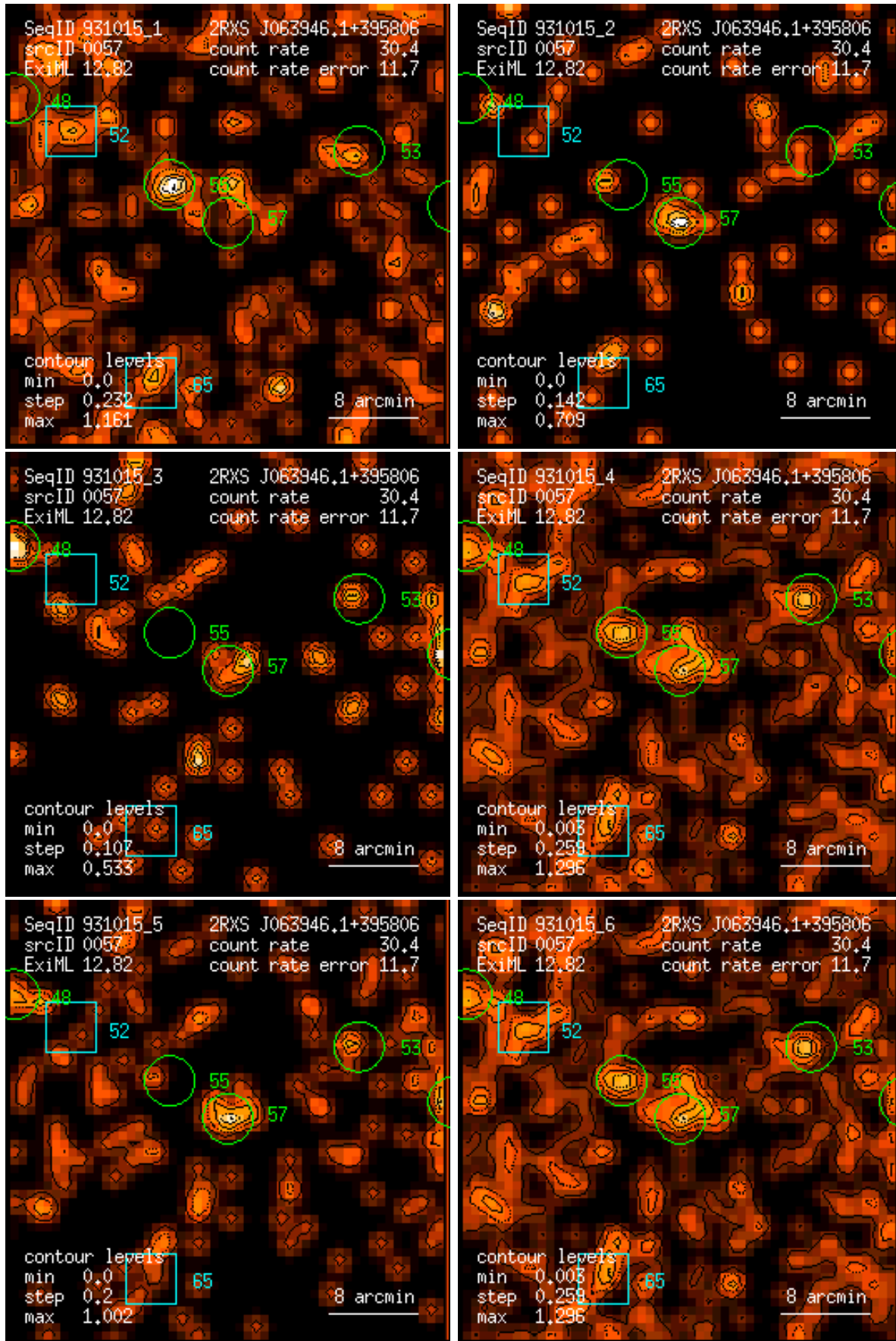
Figure 57: RASS 931015: detection 0057: band rate images, Gaussian filter: (1) PSPC channels 11 – 41, (2) 52 – 90, (3) 91 – 201, (4) 11 – 235, (5) 52 – 201, (6) 11 – 201. Broad band rates in counts/ks. Band rate contour levels in counts/ks/arcmin 2 .
