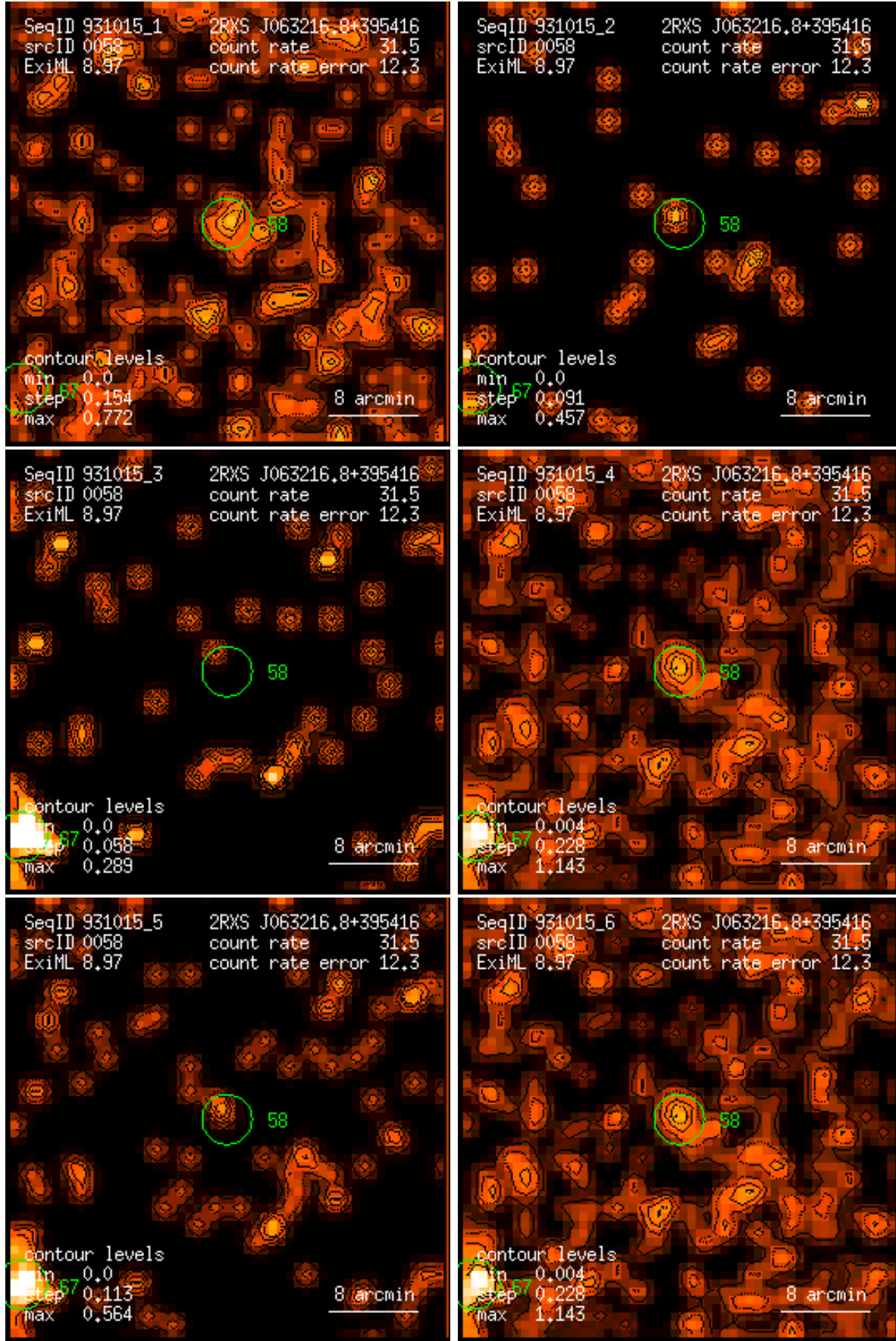
Figure 58: RASS 931015: detection 0058: band rate images, Gaussian filter: (1) PSPC channels 11 – 41, (2) 52 – 90, (3) 91 – 201, (4) 11 – 235, (5) 52 – 201, (6) 11 – 201. Broad band rates in counts/ks. Band rate contour levels in counts/ks/arcmin 2 .
