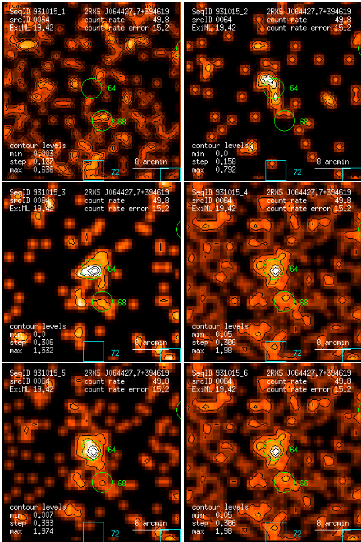
Figure 64: RASS 931015: detection 0064: band rate images, Gaussian filter: (1) PSPC channels 11 – 41, (2) 52 – 90, (3) 91 – 201, (4) 11 – 235, (5) 52 – 201, (6) 11 – 201. Broad band rates in counts/ks. Band rate contour levels in counts/ks/arcmin 2 .
