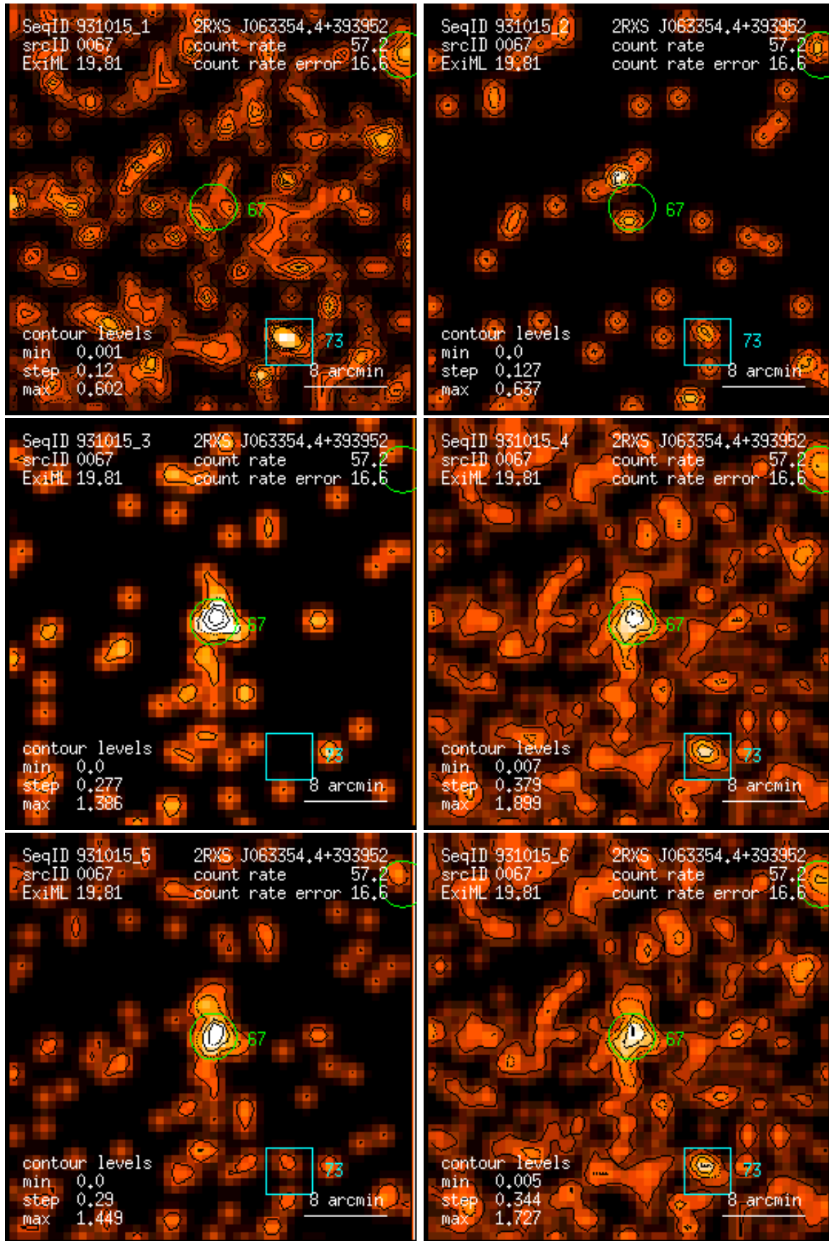
Figure 67: RASS 931015: detection 0067: band rate images, Gaussian filter: (1) PSPC channels 11 – 41, (2) 52 – 90, (3) 91 – 201, (4) 11 – 235, (5) 52 – 201, (6) 11 – 201. Broad band rates in counts/ks. Band rate contour levels in counts/ks/arcmin 2 .
