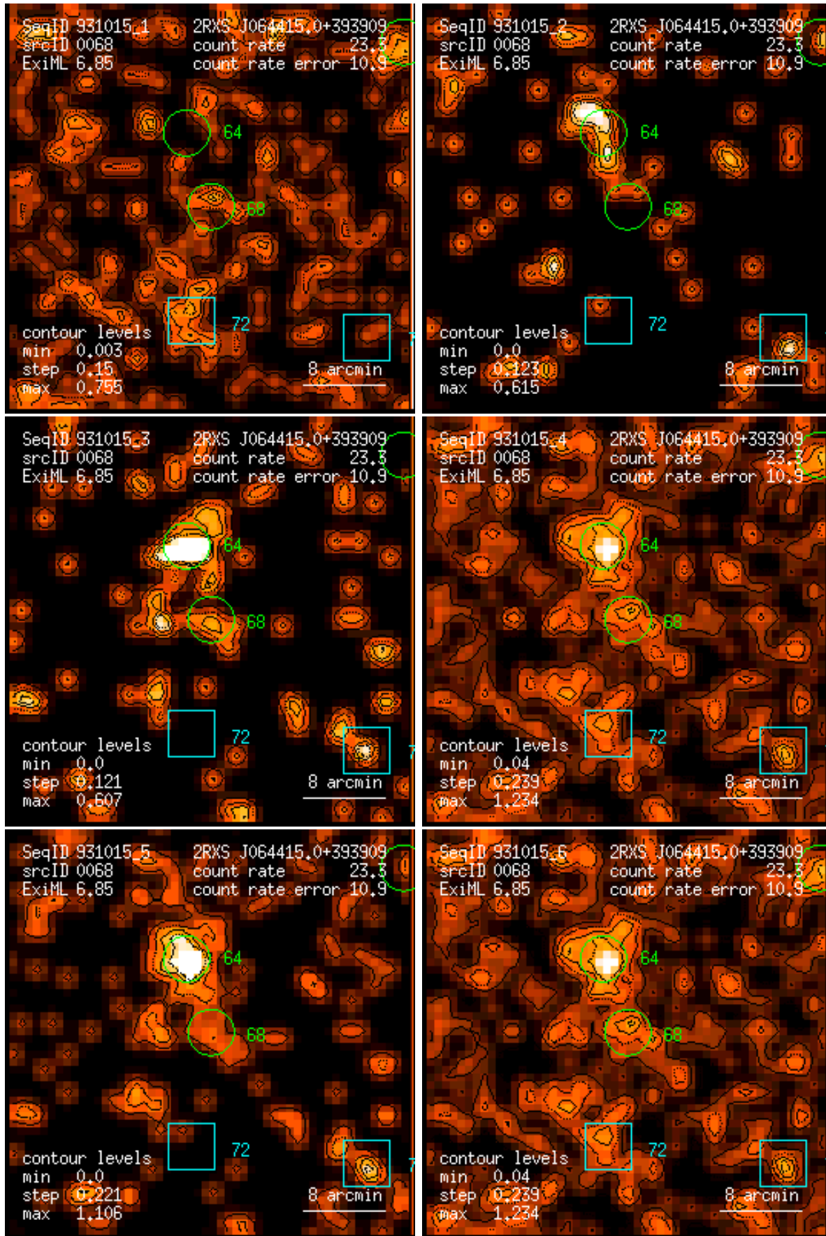
Figure 68: RASS 931015: detection 0068: band rate images, Gaussian filter: (1) PSPC channels 11 – 41, (2) 52 – 90, (3) 91 – 201, (4) 11 – 235, (5) 52 – 201, (6) 11 – 201. Broad band rates in counts/ks. Band rate contour levels in counts/ks/arcmin 2 .
