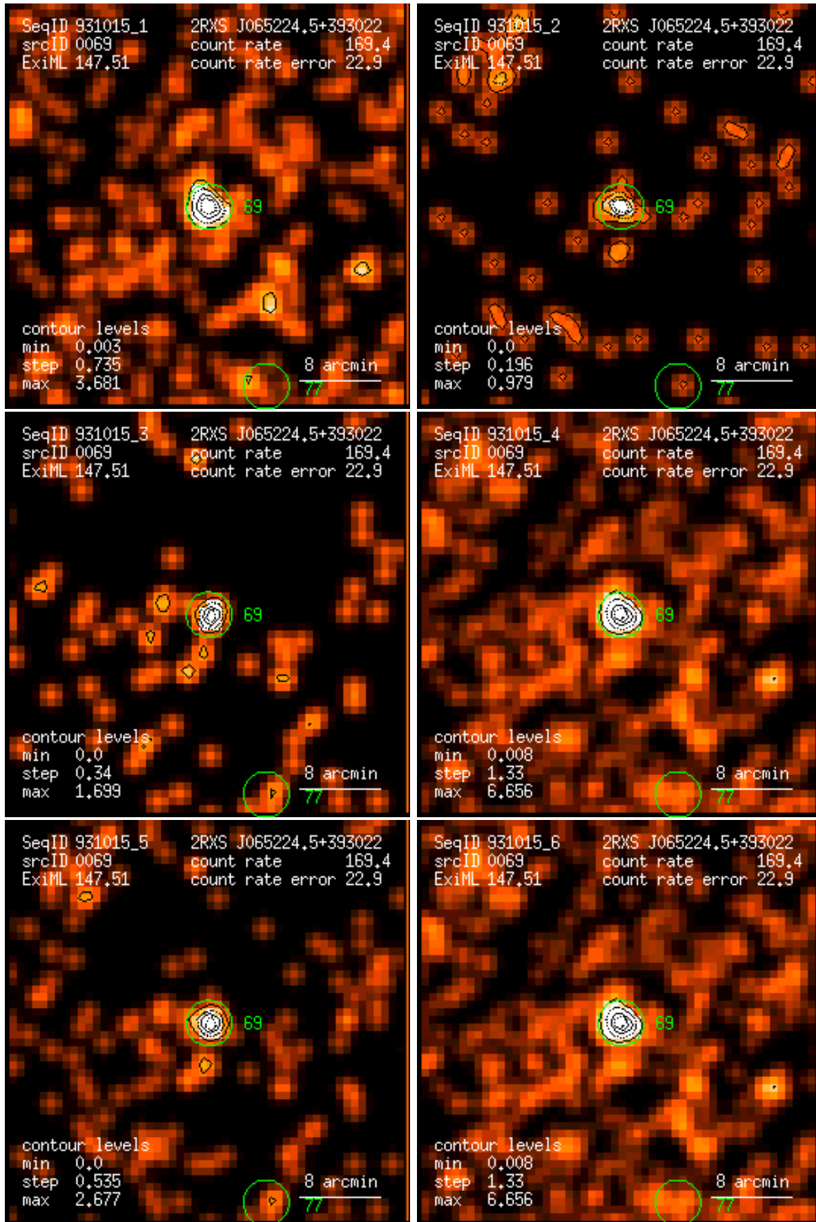
Figure 69: RASS 931015: detection 0069: band rate images, Gaussian filter: (1) PSPC channels 11 – 41, (2) 52 – 90, (3) 91 – 201, (4) 11 – 235, (5) 52 – 201, (6) 11 – 201. Broad band rates in counts/ks. Band rate contour levels in counts/ks/arcmin 2 .
