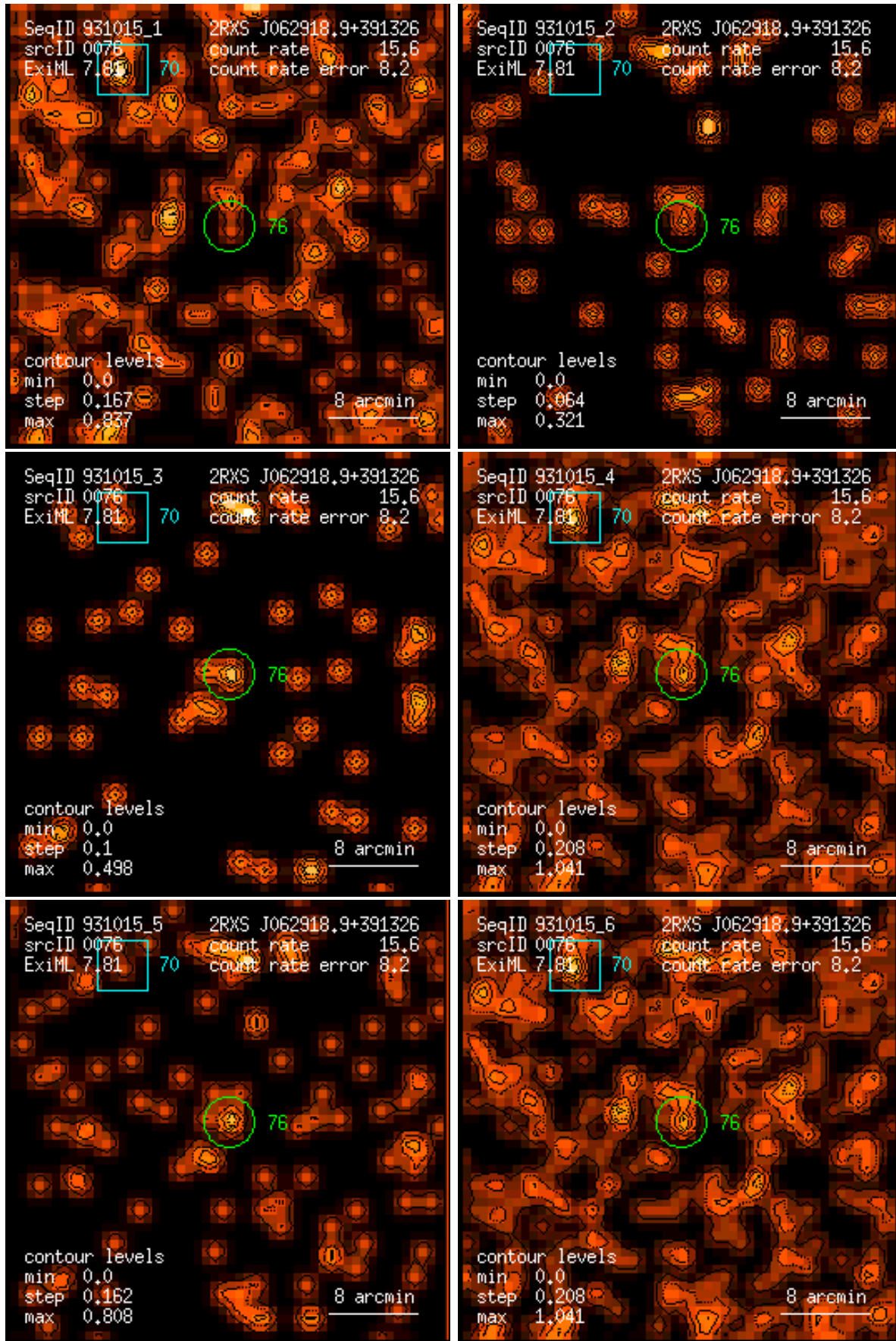
Figure 76: RASS 931015: detection 0076: band rate images, Gaussian filter: (1) PSPC channels 11 – 41, (2) 52 – 90, (3) 91 – 201, (4) 11 – 235, (5) 52 – 201, (6) 11 – 201. Broad band rates in counts/ks. Band rate contour levels in counts/ks/arcmin 2 .
