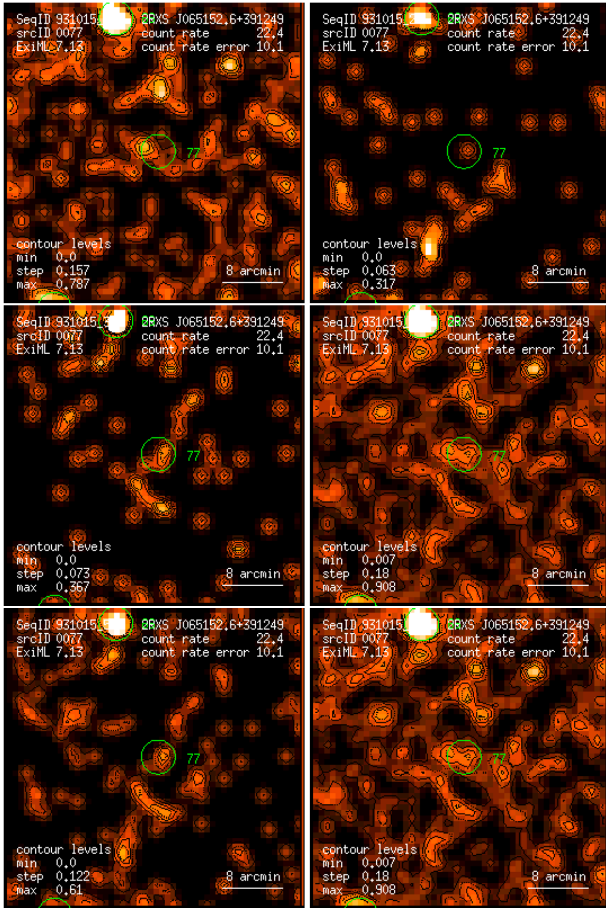
Figure 77: RASS 931015: detection 0077: band rate images, Gaussian filter: (1) PSPC channels 11 – 41, (2) 52 – 90, (3) 91 – 201, (4) 11 – 235, (5) 52 – 201, (6) 11 – 201. Broad band rates in counts/ks. Band rate contour levels in counts/ks/arcmin 2 .
