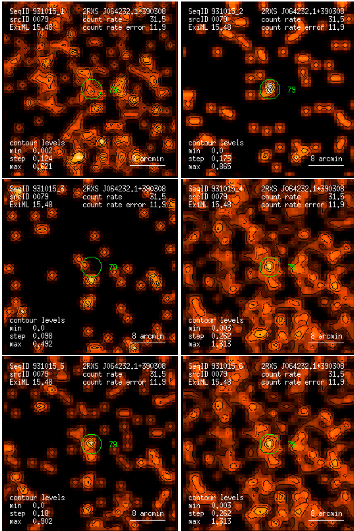
Figure 79: RASS 931015: detection 0079: band rate images, Gaussian filter: (1) PSPC channels 11 – 41, (2) 52 – 90, (3) 91 – 201, (4) 11 – 235, (5) 52 – 201, (6) 11 – 201. Broad band rates in counts/ks. Band rate contour levels in counts/ks/arcmin 2 .
