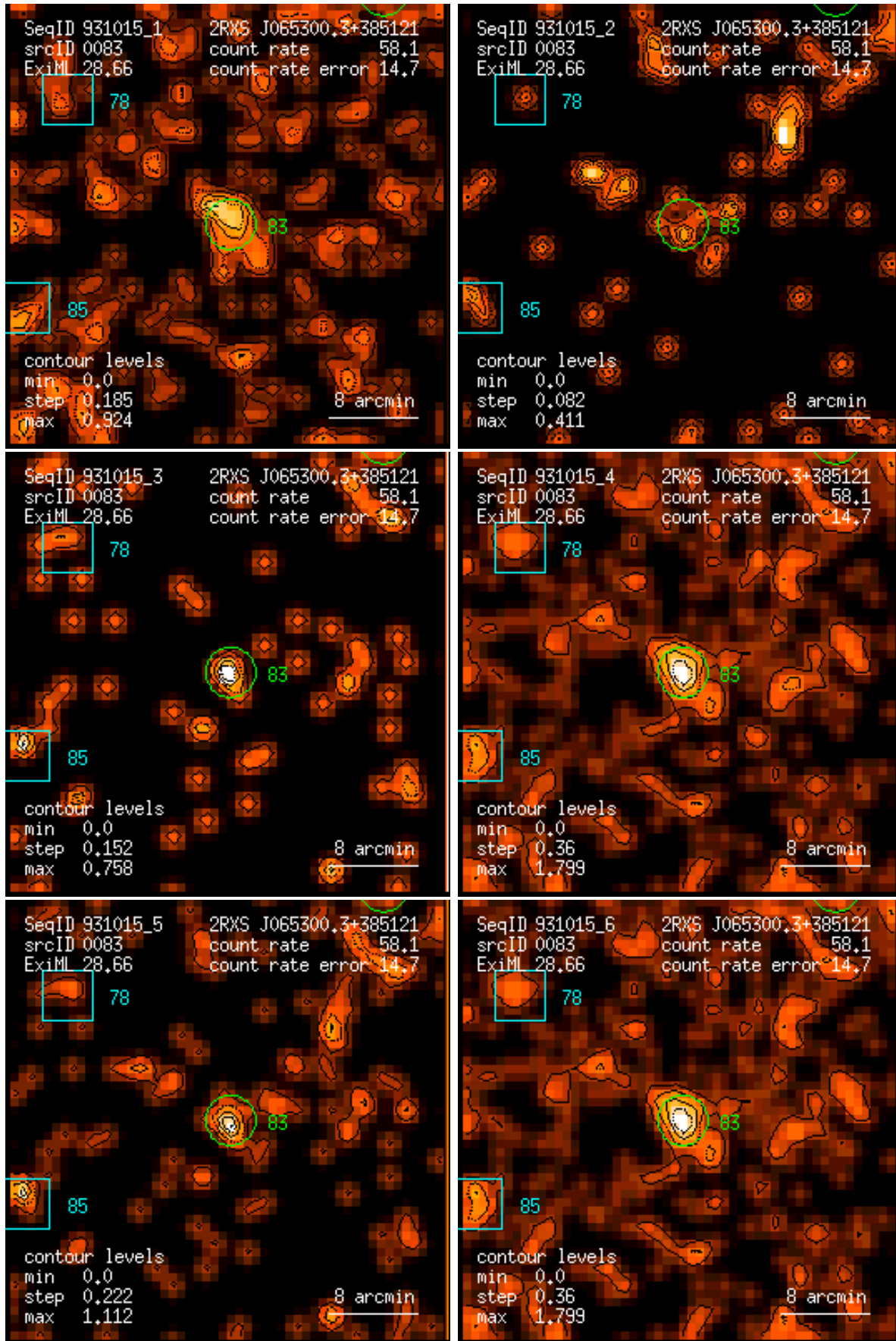
Figure 83: RASS 931015: detection 0083: band rate images, Gaussian filter: (1) PSPC channels 11 – 41, (2) 52 – 90, (3) 91 – 201, (4) 11 – 235, (5) 52 – 201, (6) 11 – 201. Broad band rates in counts/ks. Band rate contour levels in counts/ks/arcmin 2 .
