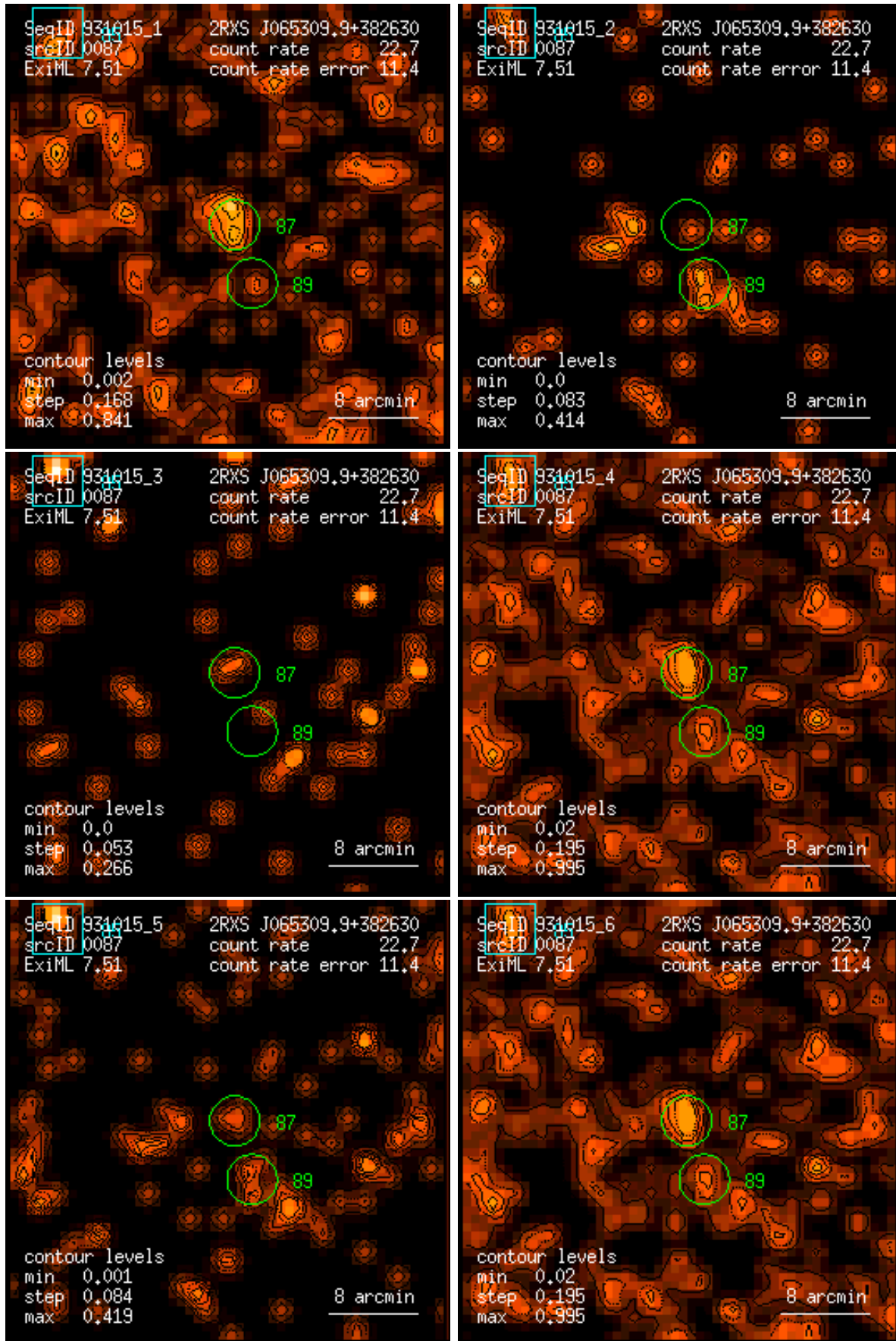
Figure 87: RASS 931015: detection 0087: band rate images, Gaussian filter: (1) PSPC channels 11 – 41, (2) 52 – 90, (3) 91 – 201, (4) 11 – 235, (5) 52 – 201, (6) 11 – 201. Broad band rates in counts/ks. Band rate contour levels in counts/ks/arcmin 2 .
