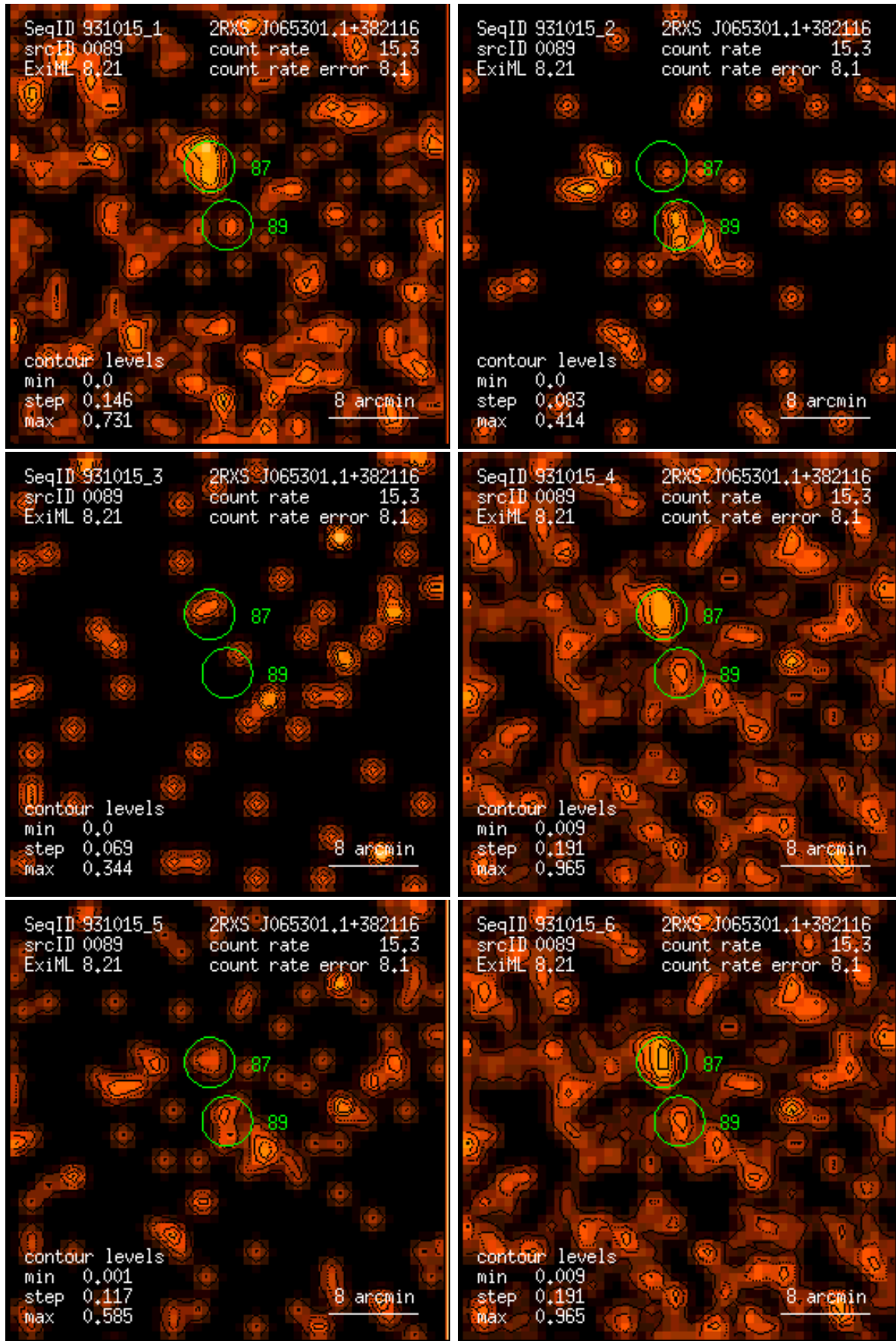
Figure 89: RASS 931015: detection 0089: band rate images, Gaussian filter: (1) PSPC channels 11 – 41, (2) 52 – 90, (3) 91 – 201, (4) 11 – 235, (5) 52 – 201, (6) 11 – 201. Broad band rates in counts/ks. Band rate contour levels in counts/ks/arcmin 2 .
