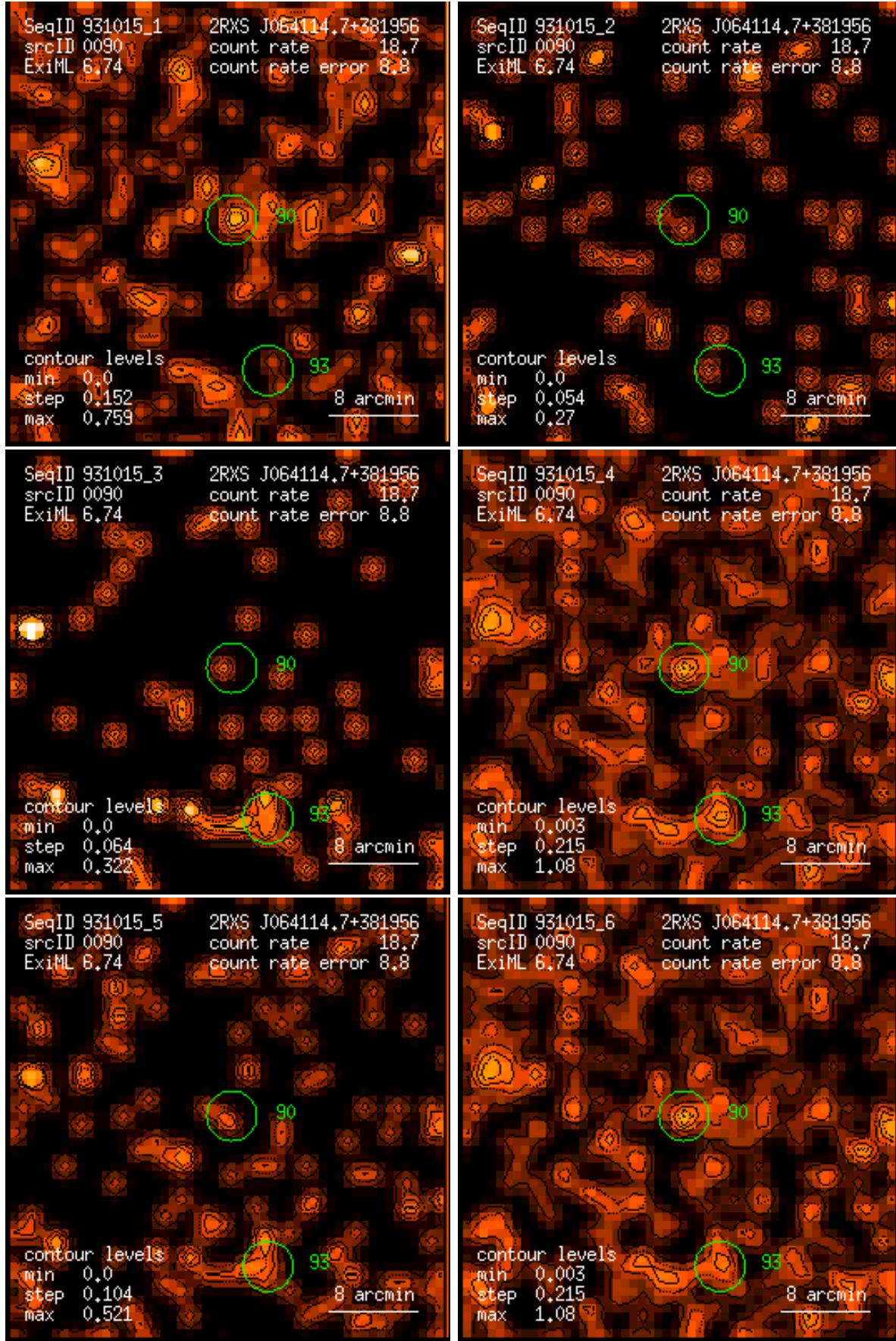
Figure 90: RASS 931015: detection 0090: band rate images, Gaussian filter: (1) PSPC channels 11 – 41, (2) 52 – 90, (3) 91 – 201, (4) 11 – 235, (5) 52 – 201, (6) 11 – 201. Broad band rates in counts/ks. Band rate contour levels in counts/ks/arcmin 2 .
