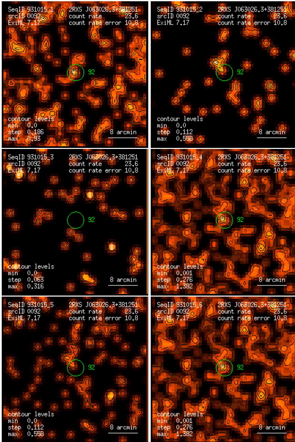
Figure 92: RASS 931015: detection 0092: band rate images, Gaussian filter: (1) PSPC channels 11 – 41, (2) 52 – 90, (3) 91 – 201, (4) 11 – 235, (5) 52 – 201, (6) 11 – 201. Broad band rates in counts/ks. Band rate contour levels in counts/ks/arcmin 2 .
