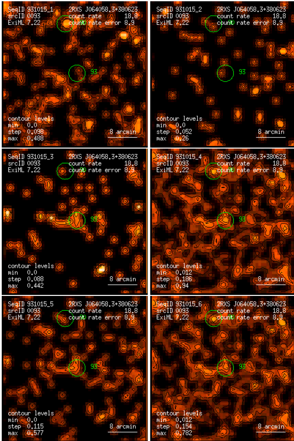
Figure 93: RASS 931015: detection 0093: band rate images, Gaussian filter: (1) PSPC channels 11 – 41, (2) 52 – 90, (3) 91 – 201, (4) 11 – 235, (5) 52 – 201, (6) 11 – 201. Broad band rates in counts/ks. Band rate contour levels in counts/ks/arcmin 2 .
