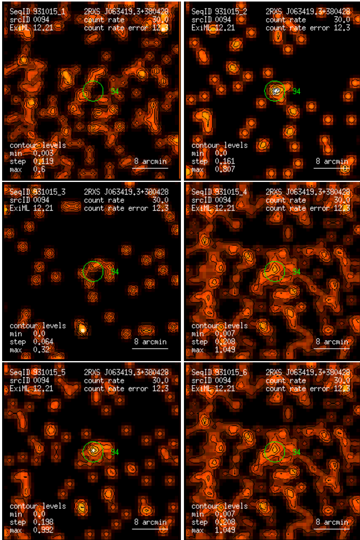
Figure 94: RASS 931015: detection 0094: band rate images, Gaussian filter: (1) PSPC channels 11 – 41, (2) 52 – 90, (3) 91 – 201, (4) 11 – 235, (5) 52 – 201, (6) 11 – 201. Broad band rates in counts/ks. Band rate contour levels in counts/ks/arcmin 2 .
