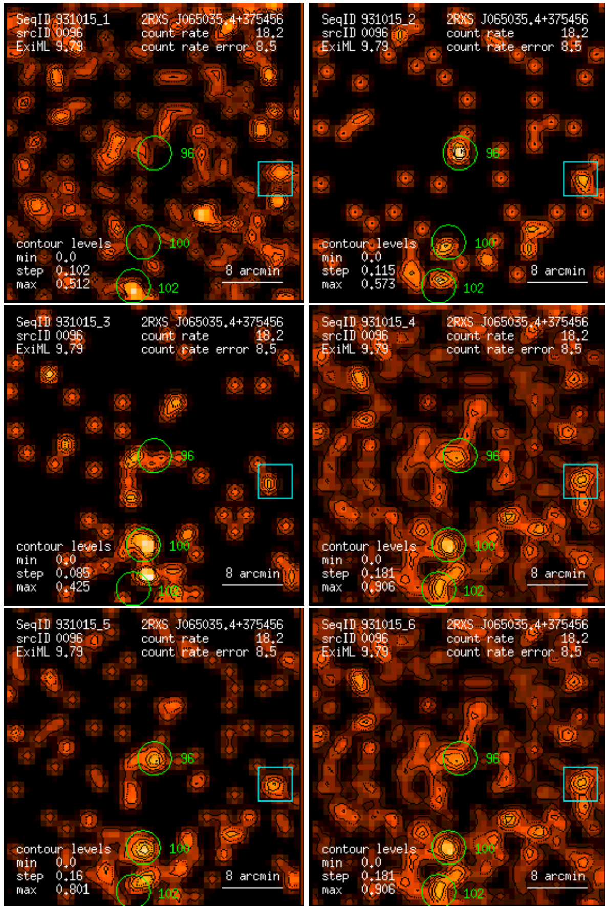
Figure 96: RASS 931015: detection 0096: band rate images, Gaussian filter: (1) PSPC channels 11 – 41, (2) 52 – 90, (3) 91 – 201, (4) 11 – 235, (5) 52 – 201, (6) 11 – 201. Broad band rates in counts/ks. Band rate contour levels in counts/ks/arcmin 2 .
