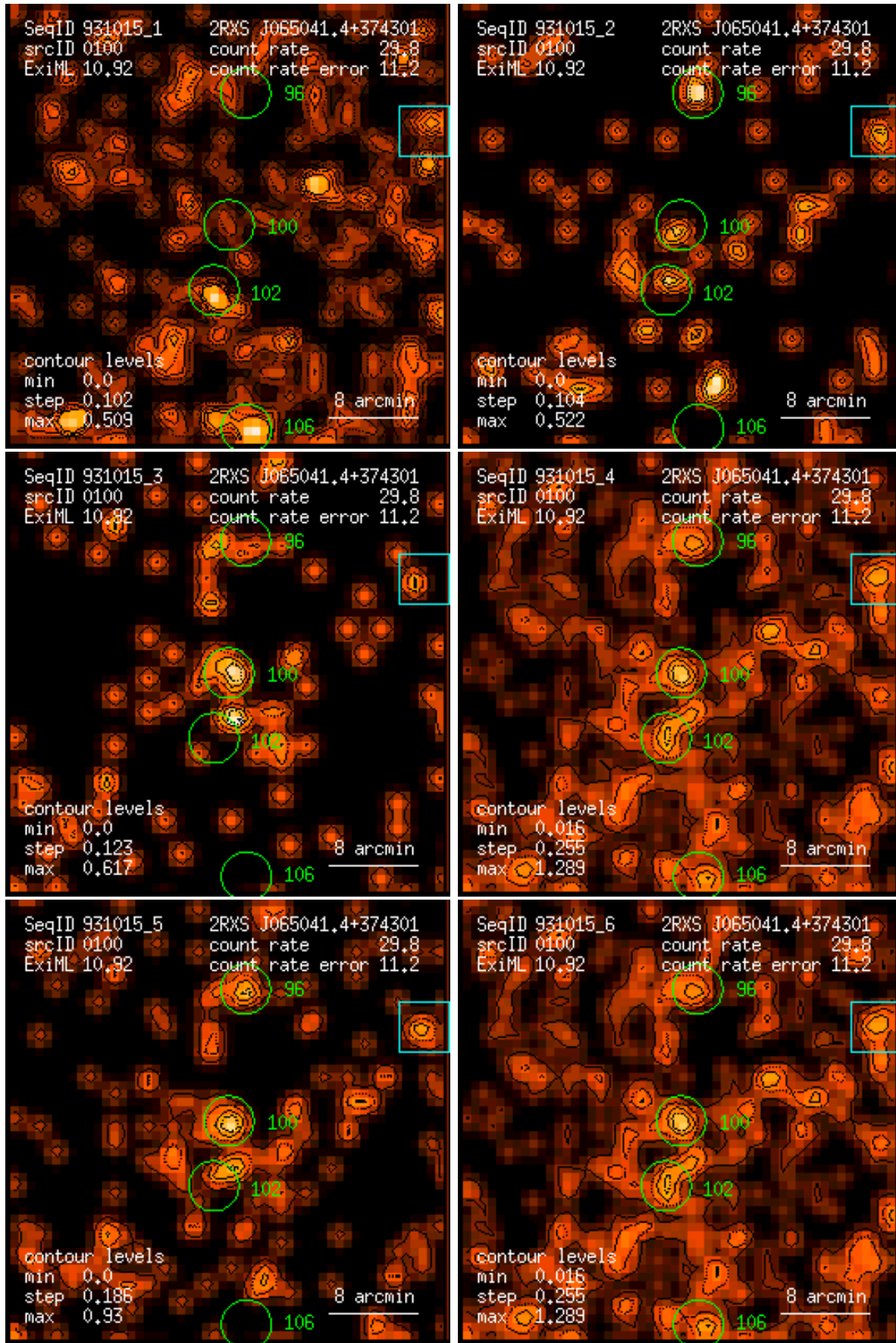
Figure 100: RASS 931015: detection 0100: band rate images, Gaussian filter: (1) PSPC channels 11 – 41, (2) 52 – 90, (3) 91 – 201, (4) 11 – 235, (5) 52 – 201, (6) 11 – 201. Broad band rates in counts/ks. Band rate contour levels in counts/ks/arcmin 2 .
