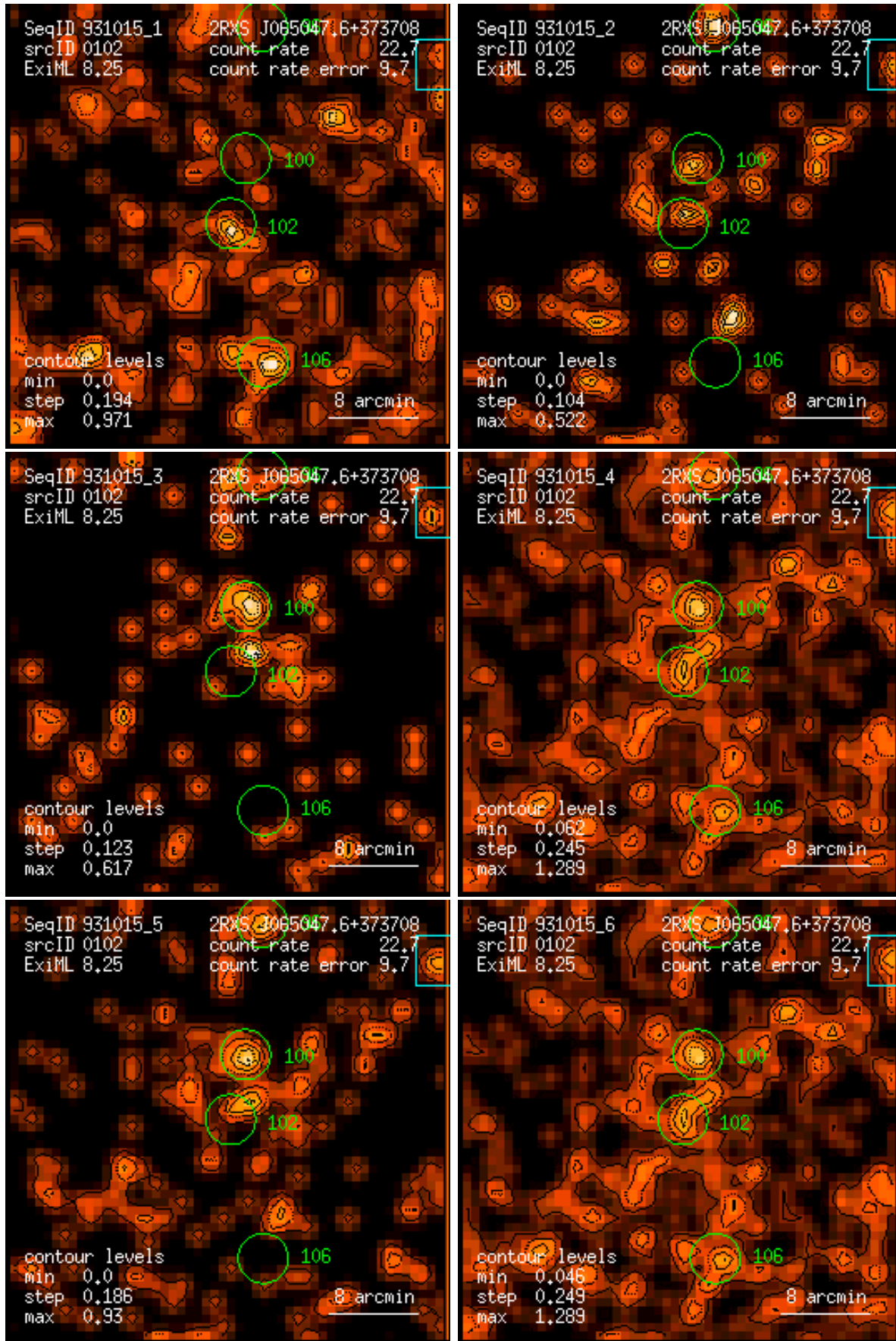
Figure 102: RASS 931015: detection 0102: band rate images, Gaussian filter: (1) PSPC channels 11 – 41, (2) 52 – 90, (3) 91 – 201, (4) 11 – 235, (5) 52 – 201, (6) 11 – 201. Broad band rates in counts/ks. Band rate contour levels in counts/ks/arcmin 2 .
