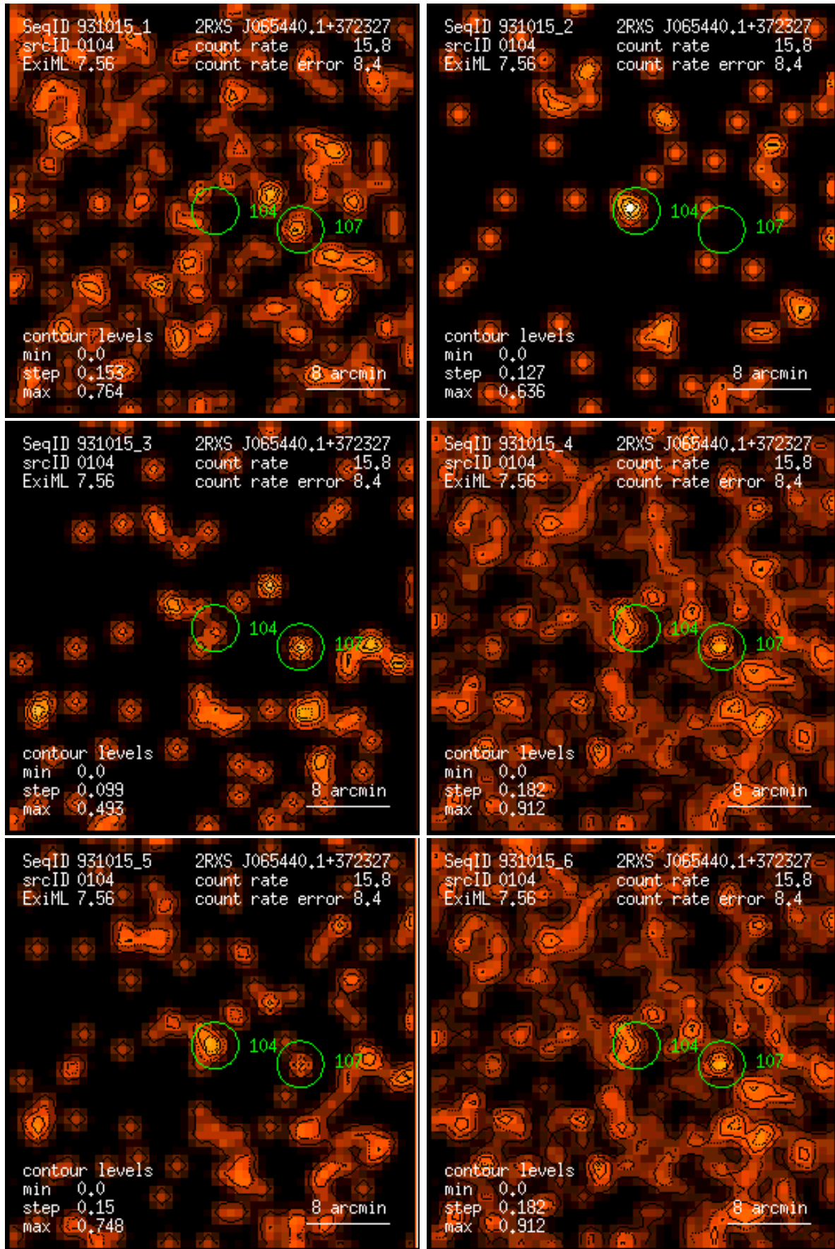
Figure 104: RASS 931015: detection 0104: band rate images, Gaussian filter: (1) PSPC channels 11 – 41, (2) 52 – 90, (3) 91 – 201, (4) 11 – 235, (5) 52 – 201, (6) 11 – 201. Broad band rates in counts/ks. Band rate contour levels in counts/ks/arcmin 2 .
