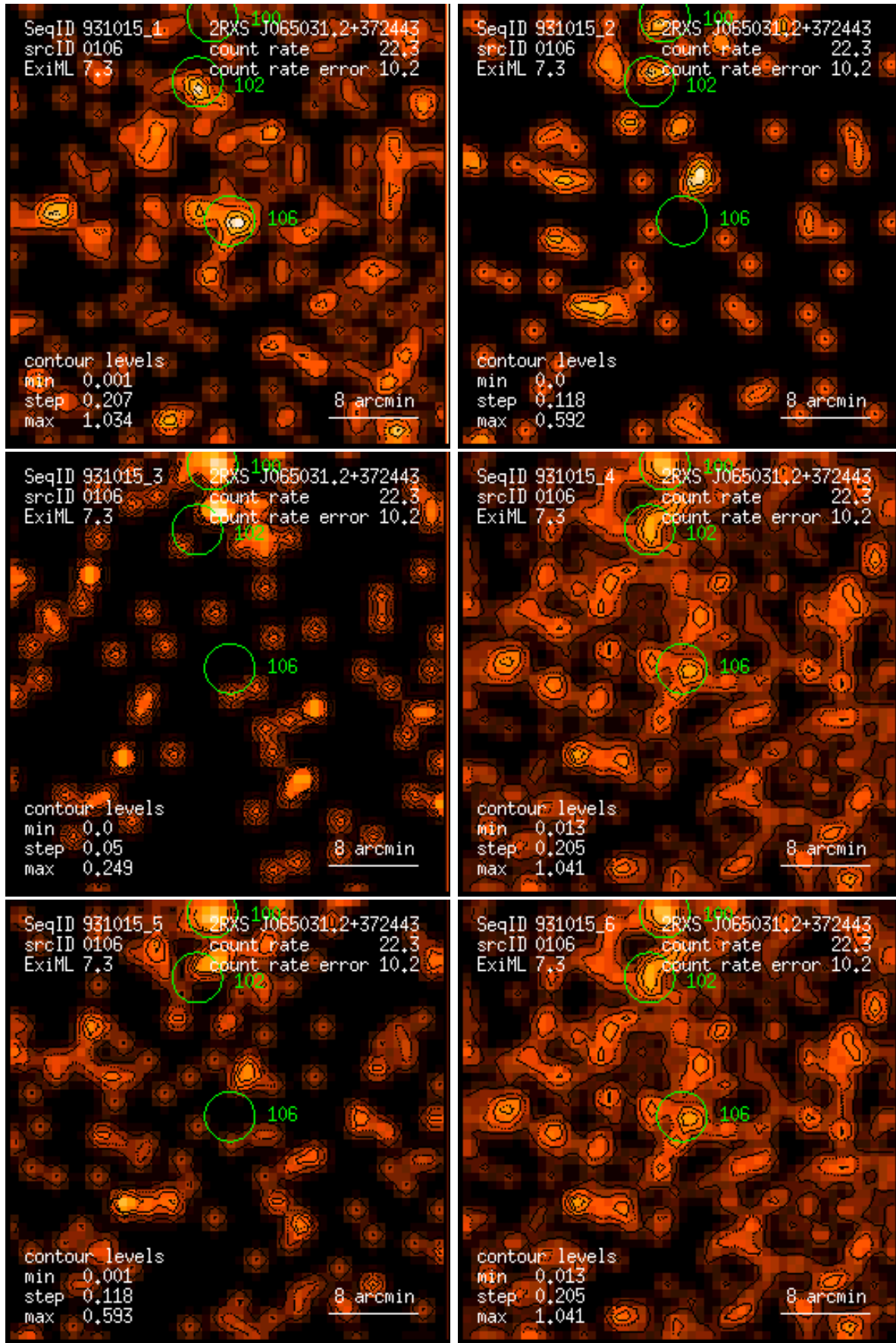
Figure 106: RASS 931015: detection 0106: band rate images, Gaussian filter: (1) PSPC channels 11 – 41, (2) 52 – 90, (3) 91 – 201, (4) 11 – 235, (5) 52 – 201, (6) 11 – 201. Broad band rates in counts/ks. Band rate contour levels in counts/ks/arcmin 2 .
