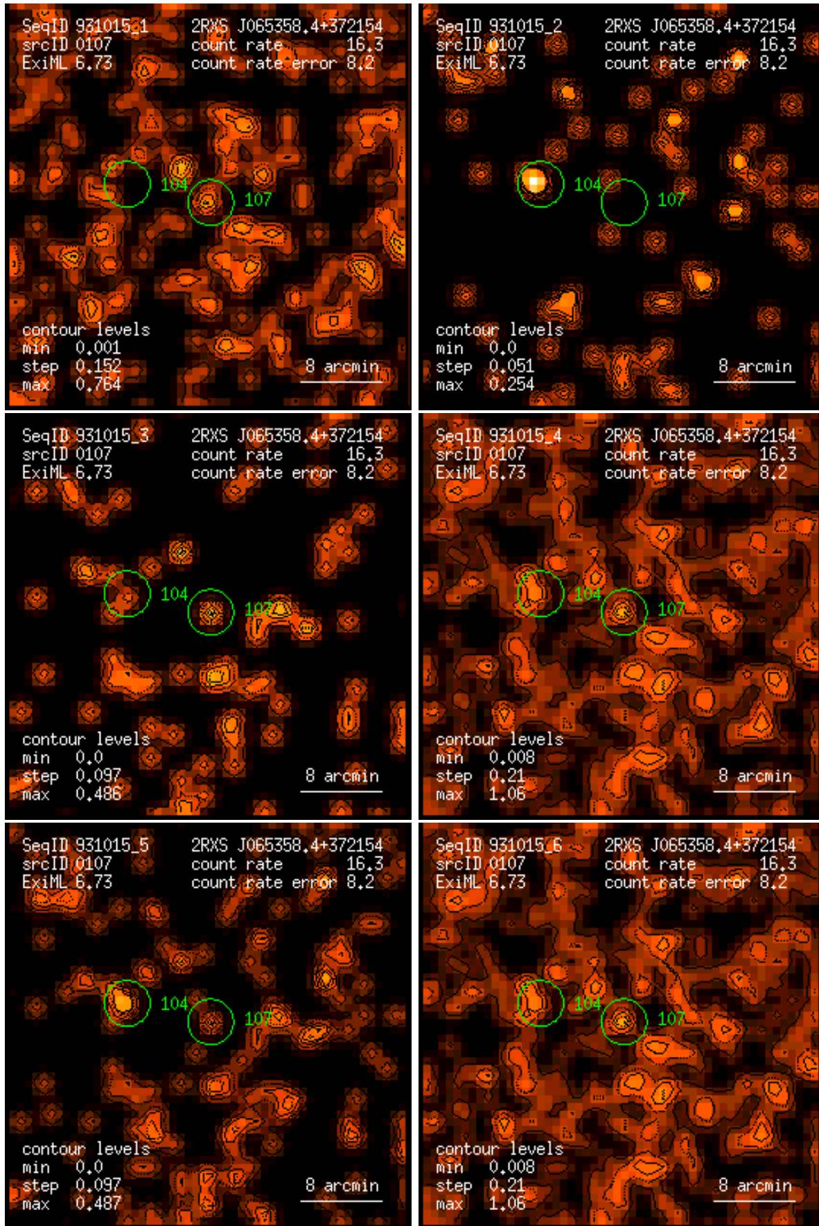
Figure 107: RASS 931015: detection 0107: band rate images, Gaussian filter: (1) PSPC channels 11 – 41, (2) 52 – 90, (3) 91 – 201, (4) 11 – 235, (5) 52 – 201, (6) 11 – 201. Broad band rates in counts/ks. Band rate contour levels in counts/ks/arcmin 2 .
